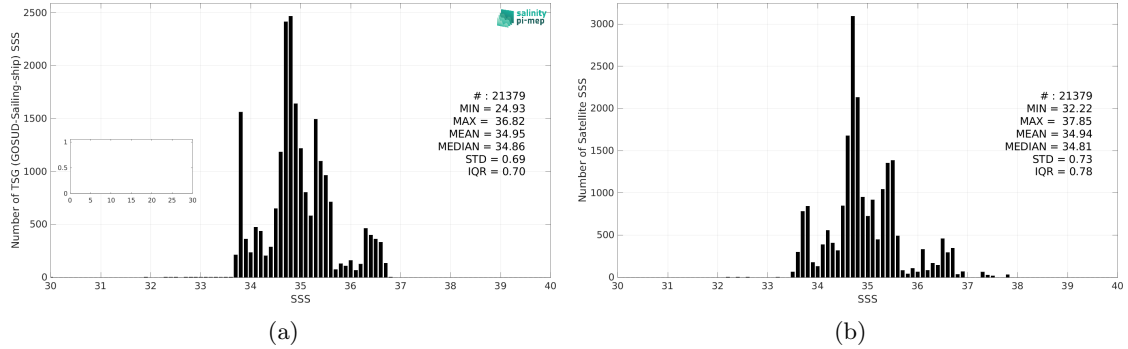
Figure 3: Histograms of SSS from TSG (GOSUD-Sailing-ship) (a) and CCI SSS L4 Merged-OI v4.41 - 30-day running (ESA) (b) considering all match-up pairs per bins of 0.1 over the Indian Ocean Pi-MEP region and for the full satellite product period.
