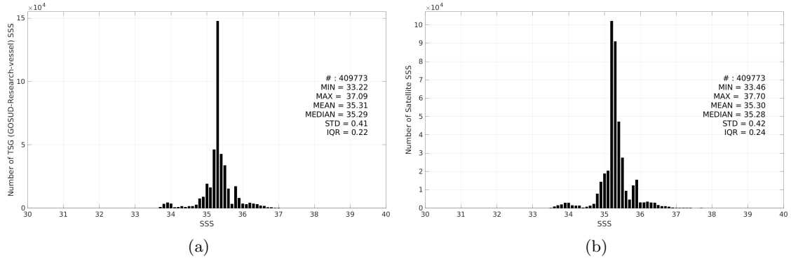
Figure 3: Histograms of SSS from TSG (GOSUD-Research-vessel) (a) and CCI SSS L4 Merged-OI v4.41 - 30-day running (ESA) (b) considering all match-up pairs per bins of 0.1 over the Indian Ocean Pi-MEP region and for the full satellite product period.
