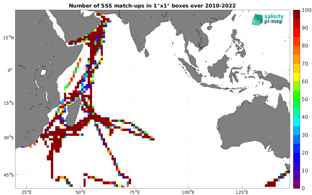
Figure 5: Number of SSS match-ups between TSG (GOSUD-Research-vessel) SSS and the CCI SSS L4 Merged-OI v4.41 - 30-day running (ESA) SSS product for the Indian Ocean Pi-MEP region over 1^\circ \times 1^\circ boxes and for the full satellite product period.
