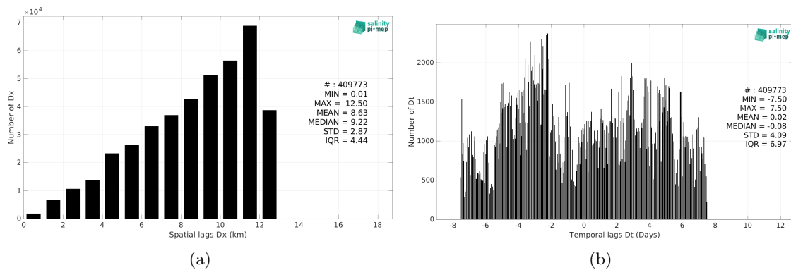
Figure 6: Histograms of the spatial (a) and temporal (b) lags between the location/time of the TSG (GOSUD-Research-vessel) measurement and the date of the corresponding CCI SSS L4 Merged-OI v4.41 - 30-day running (ESA) SSS pixel.
