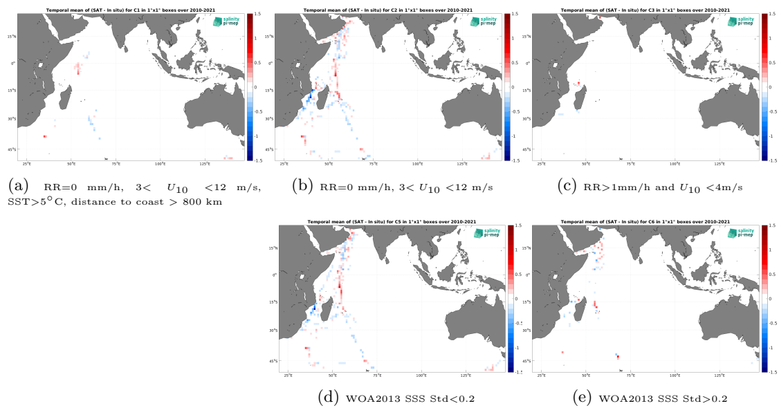
Figure 14: Temporal mean gridded over spatial boxes of size 1^\circ \times 1^\circ of \Delta SSS (CCI SSS L4 Merged-OI v4.41 - 30-day running (ESA) - TSG (GOSUD-Research-vessel)) for 5 different subdatasets corresponding to:RR=0 mm/h, 3 < U_{10} < 12 m/s, SST >5^\circ C, distance to coast > 800 km (a), RR=0 mm/h, 3 < U_{10} < 12 m/s (b), RR >1 mm/h and U_{10} < 4 m/s (c), WOA2013 SSS Std <0.2 (d), WOA2013 SSS Std >0.2 (e).
