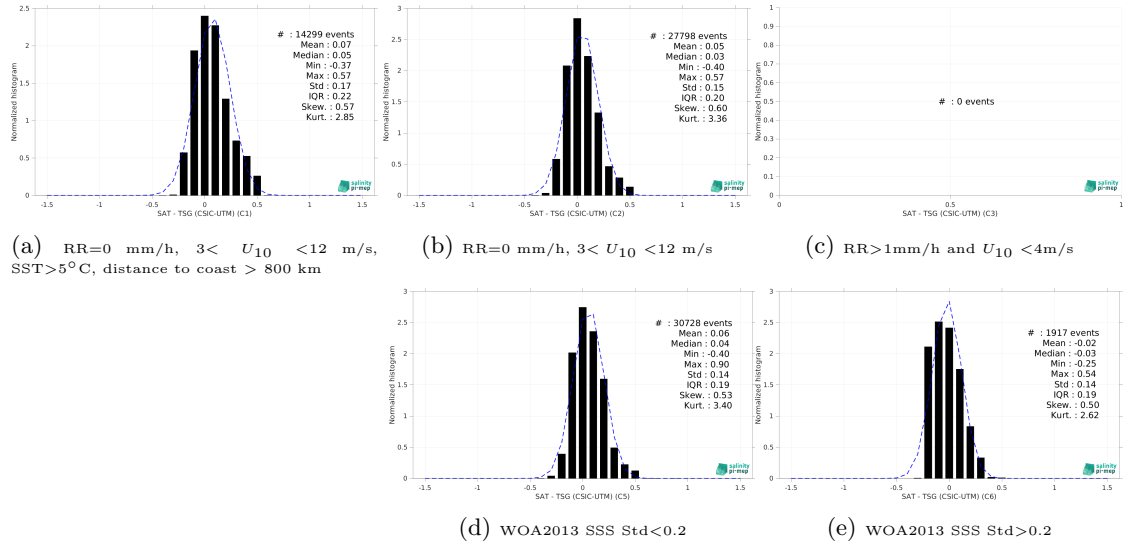
Figure 15: Normalized histogram of \Delta SSS (CCI SSS L4 Merged-OI v4.41 - 30-day running (ESA) - TSG (CSIC-UTM)) for 5 different subdatasets corresponding to: RR=0 mm/h, 3 < U_{10} < 12 m/s, SST > 5°C, distance to coast > 800 km (a), RR=0 mm/h, 3 < U_{10} < 12 m/s (b), RR > 1mm/h and U_{10} < 4 m/s (c), WOA2013 SSS Std < 0.2 (d), WOA2013 SSS Std > 0.2 (e).
