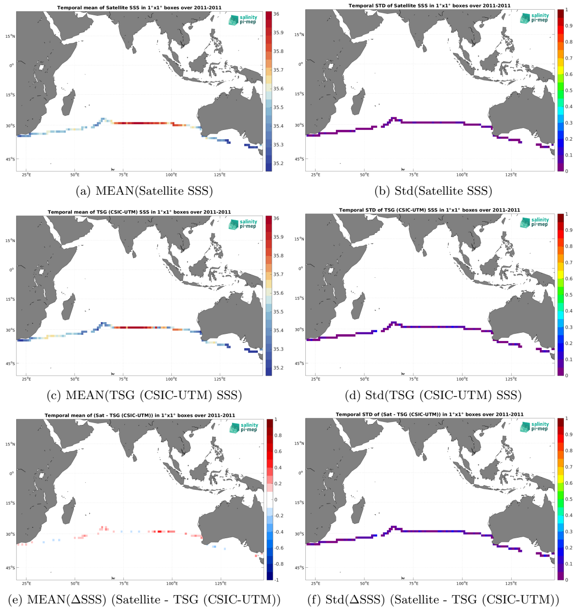
Figure 7: Temporal mean (left) and Std (right) of SSS from CCI SSS L4 Merged-OI v4.41 - 30-day running (ESA) (top), TSG (CSIC-UTM) (middle), and of \Delta SSS (Satellite - TSG (CSIC-UTM)). Only match-up pairs are used to generate these maps.
