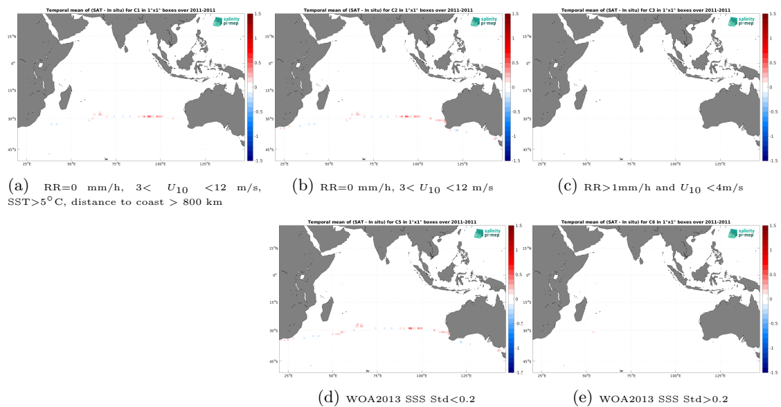
Figure 14: Temporal mean gridded over spatial boxes of size 1^\circ \times 1^\circ of \Delta SSS (CCI SSS L4 Merged-OI v4.41 - 30-day running (ESA) - TSG (CSIC-UTM)) for 5 different subdatasets corresponding to: RR=0 mm/h, 3 < U_{10} < 12 m/s, SST > 5^\circ\text{C} , distance to coast > 800 km (a), RR=0 mm/h, 3 < U_{10} < 12 m/s (b), RR > 1 mm/h and U_{10} < 4 m/s (c), WOA2013 SSS Std < 0.2 (d), WOA2013 SSS Std > 0.2 (e).
