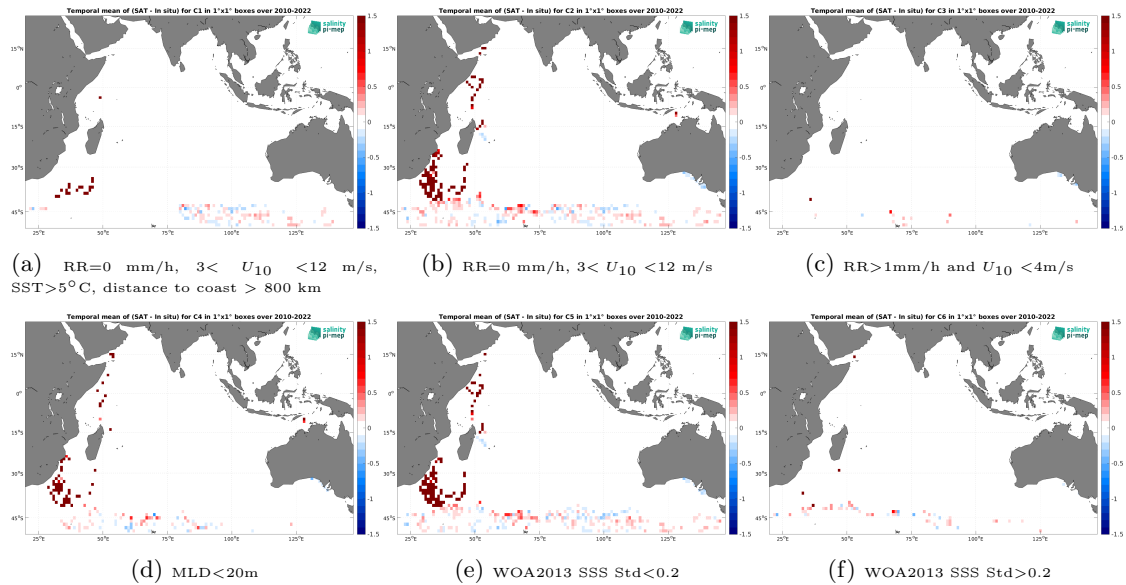
Figure 14: Temporal mean gridded over spatial boxes of size 1^\circ \times 1^\circ of \Delta\text{SSS} (CCI SSS L4 Merged-OI v4.41 - 30-day running (ESA) - Marine mammals) for 6 different subdatasets corresponding to: RR=0 mm/h, 3 < U_{10} < 12 m/s, SST > 5°C, distance to coast > 800 km (a), RR=0 mm/h, 3 < U_{10} < 12 m/s (b), RR > 1mm/h and U_{10} < 4 m/s (c), MLD < 20m (d), WOA2013 SSS Std < 0.2 (e), WOA2013 SSS Std > 0.2 (f).
