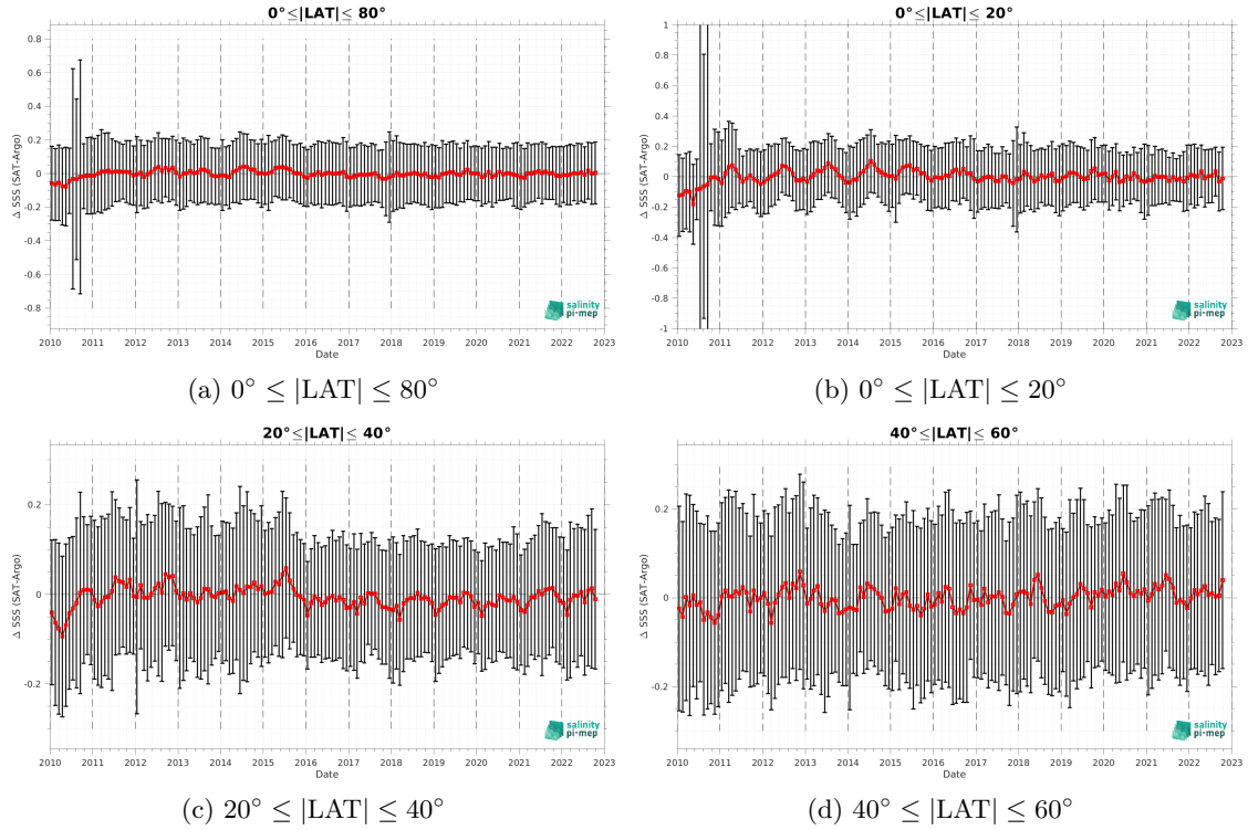
Figure 11: Monthly median (red curves) of \Delta SSS (Satellite - Argo) and \pm 1 Std (black vertical thick bars) as function of time for all the collected Pi-MEP match-up pairs estimated over the Indian Ocean Pi-MEP region and for the full satellite product period are shown for different latitude bands: (a) 80°S-80°N, (b) 20°S-20°N, (c) 40°S-20°S and 20°N-40°N and (d) 60°S-40°S and 40°N-60°N.
