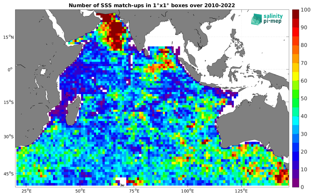
Figure 5: Number of SSS match-ups between Argo SSS and the CCI SSS L4 Merged-OI v4.41 - 30-day running (ESA) SSS product for the Indian Ocean Pi-MEP region over 1^\circ \times 1^\circ boxes and for the full satellite product period.
