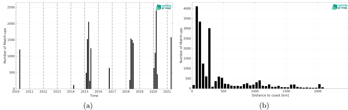
Figure 1: Number of match-ups between TSG (SAMOS) and CCI SSS L4 Merged-OI v4.4 - 7-day running (ESA) SSS as a function of time (a) and as function of the distance to coast (b) over the Indian Ocean Pi-MEP region and for the full satellite product period.
