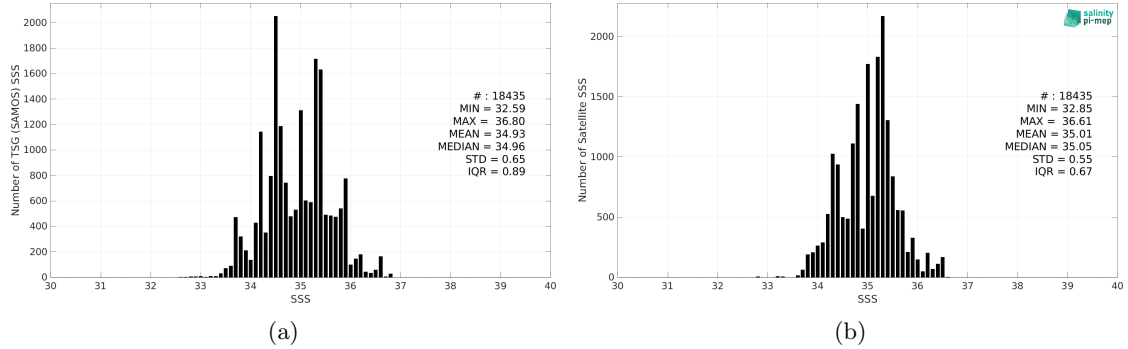
Figure 2: Histograms of SSS from TSG (SAMOS) (a) and CCI SSS L4 Merged-OI v4.4 - 7-day running (ESA) (b) considering all match-up pairs per bins of 0.1 over the Indian Ocean Pi-MEP region and for the full satellite product period.
