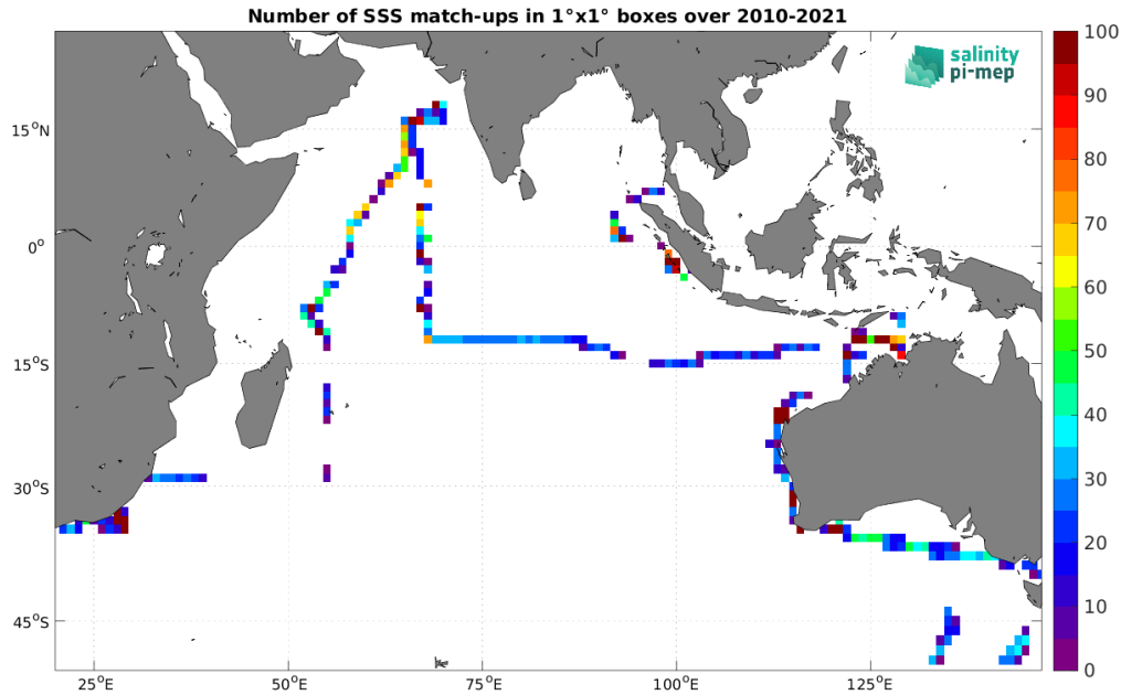
Figure 4: Number of SSS match-ups between TSG (SAMOS) SSS and the CCI SSS L4 Merged-OI v4.4 - 7-day running (ESA) SSS product for the Indian Ocean Pi-MEP region over 1°x1° boxes and for the full satellite product period.
