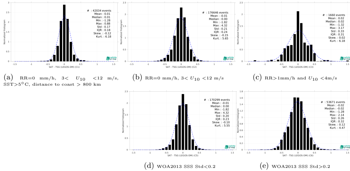
Figure 13: Normalized histogram of \Delta SSS (CCI SSS L4 Merged-OI v4.4 - 7-day running (ESA) - TSG (LEGOS-DM)) for 5 different subdatasets corresponding to: RR=0 mm/h, 3 < U_{10} < 12 m/s, SST>5°C, distance to coast > 800 km (a), RR=0 mm/h, 3 < U_{10} < 12 m/s (b), RR>1mm/h and U_{10} < 4 m/s (c), WOA2013 SSS Std<0.2 (d), WOA2013 SSS Std>0.2 (e).
