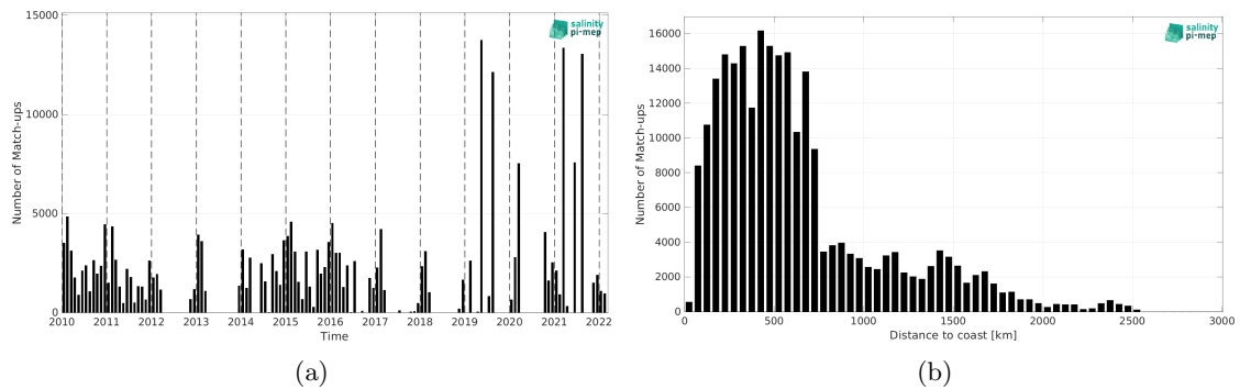
Figure 1: Number of match-ups between TSG (LEGOS-DM) and CCI SSS L4 Merged-OI v4.4 - 7-day running (ESA) SSS as a function of time (a) and as function of the distance to coast (b) over the Indian Ocean Pi-MEP region and for the full satellite product period.
