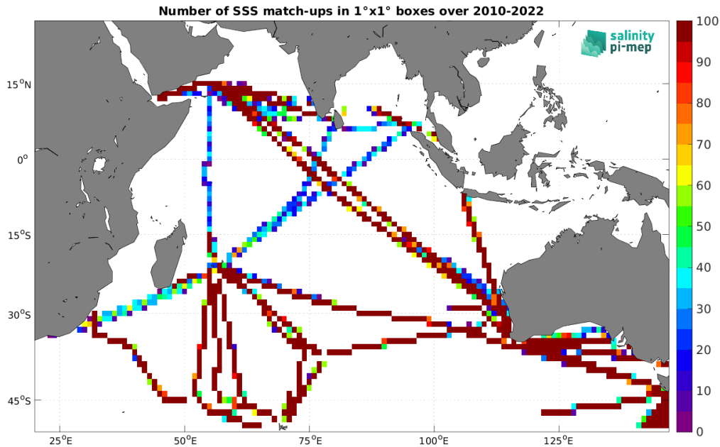
Figure 4: Number of SSS match-ups between TSG (LEGOS-DM) SSS and the CCI SSS L4 Merged-OI v4.4 - 7-day running (ESA) SSS product for the Indian Ocean Pi-MEP region over 1^\circ \times 1^\circ boxes and for the full satellite product period.
