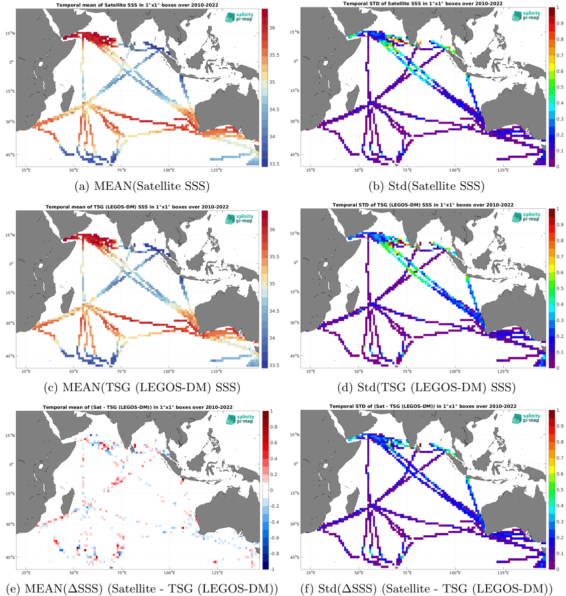
Figure 6: Temporal mean (left) and Std (right) of SSS from CCI SSS L4 Merged-OI v4.4 - 7-day running (ESA) (top), TSG (LEGOS-DM) (middle), and of \Delta SSS (Satellite - TSG (LEGOS-DM)). Only match-up pairs are used to generate these maps.
