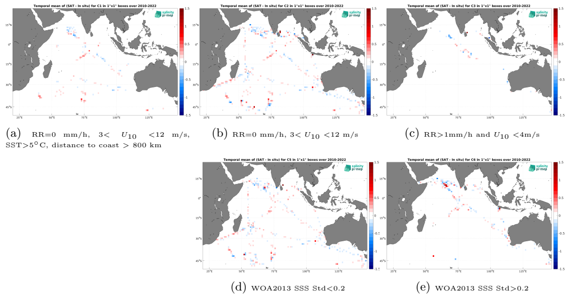
Figure 12: Temporal mean gridded over spatial boxes of size 1^\circ \times 1^\circ of \Delta SSS (CCI SSS L4 Merged-OI v4.4 - 7-day running (ESA) - TSG (LEGOS-DM)) for 5 different subdatasets corresponding to: RR=0 mm/h, 3 < U_{10} < 12 m/s, SST > 5^\circ\text{C} , distance to coast > 800 km (a), RR=0 mm/h, 3 < U_{10} < 12 m/s (b), RR > 1\text{mm/h} and U_{10} < 4\text{m/s} (c), WOA2013 SSS Std < 0.2 (d), WOA2013 SSS Std > 0.2 (e).
