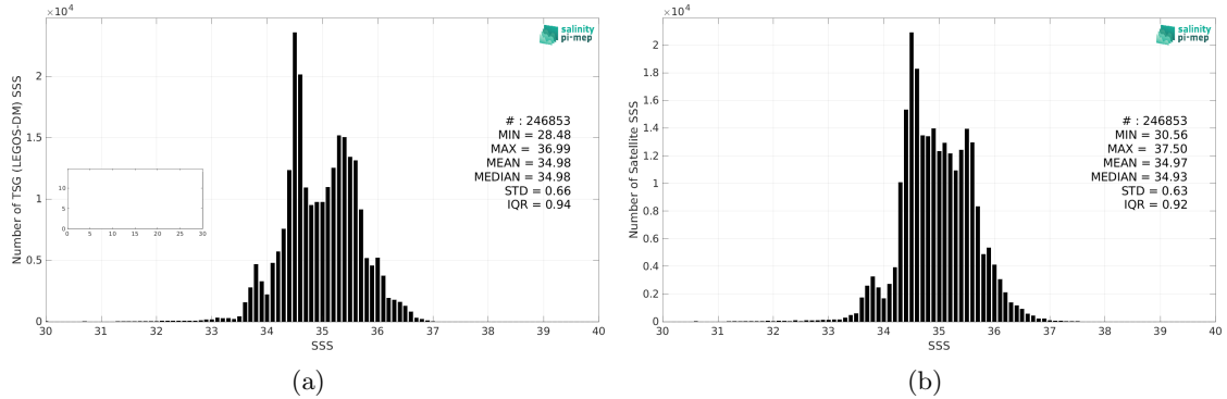
Figure 2: Histograms of SSS from TSG (LEGOS-DM) (a) and CCI SSS L4 Merged-OI v4.4 - 7-day running (ESA) (b) considering all match-up pairs per bins of 0.1 over the Indian Ocean Pi-MEP region and for the full satellite product period.
