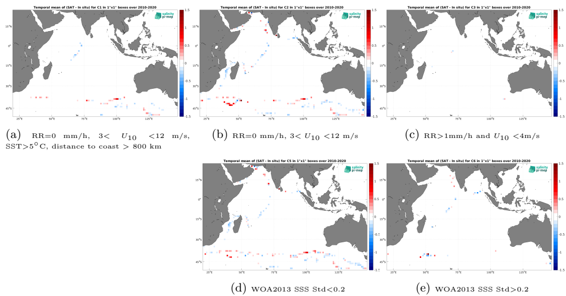
Figure 12: Temporal mean gridded over spatial boxes of size 1^\circ \times 1^\circ of \Delta SSS (CCI SSS L4 Merged-OI v4.4 - 7-day running (ESA) - TSG (GOSUD-Sailing-ship)) for 5 different subdatasets corresponding to:RR=0 mm/h, 3 < U_{10} < 12 m/s, SST >5^\circ\text{C} , distance to coast > 800 km (a), RR=0 mm/h, 3 < U_{10} < 12 m/s (b), RR >1 mm/h and U_{10} < 4 m/s (c), WOA2013 SSS Std <0.2 (d), WOA2013 SSS Std >0.2 (e).
