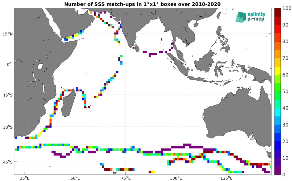
Figure 4: Number of SSS match-ups between TSG (GOSUD-Sailing-ship) SSS and the CCI SSS L4 Merged-OI v4.4 - 7-day running (ESA) SSS product for the Indian Ocean Pi-MEP region over 1^\circ \times 1^\circ boxes and for the full satellite product period.
