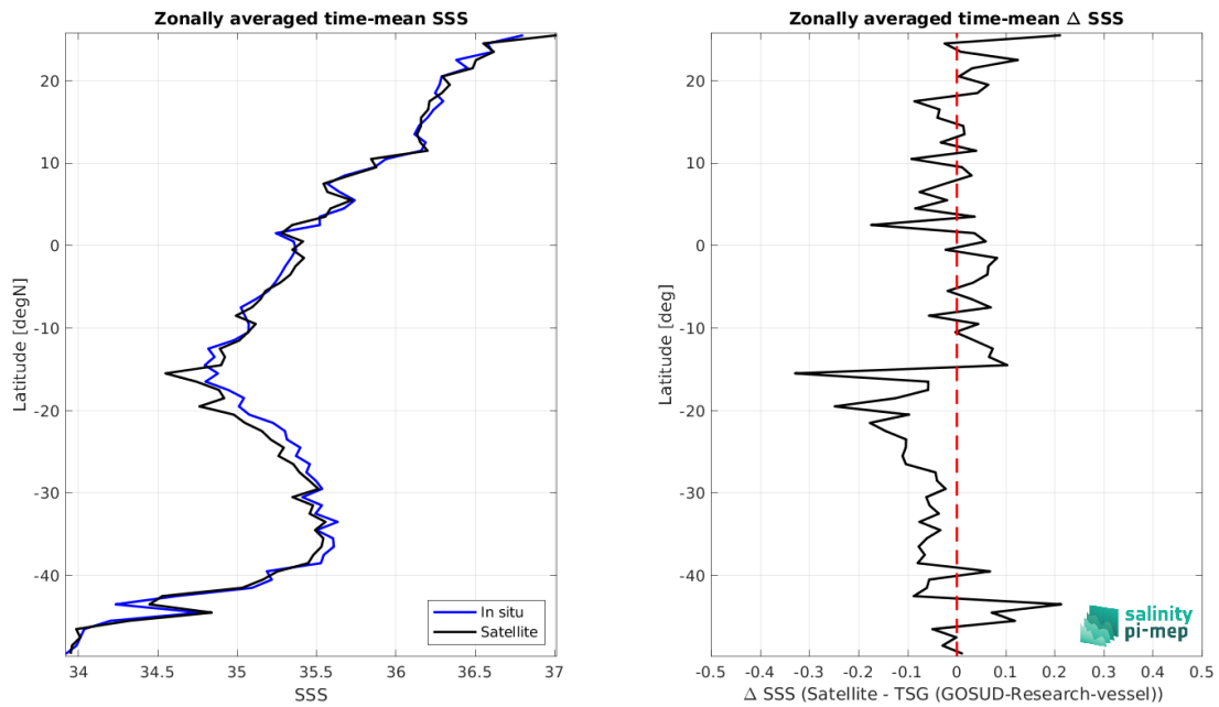
Figure 8: Left panel: Zonal mean SSS from CCI SSS L4 Merged-OI v4.4 - 7-day running (ESA) satellite product (black) and from TSG (GOSUD-Research-vessel) (blue). Right panel: Zonal mean of \Delta SSS (Satellite - TSG (GOSUD-Research-vessel)) for all the collected Pi-MEP match-up pairs estimated over the full satellite product period.
