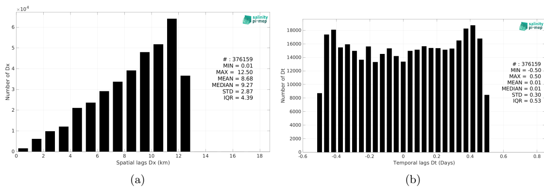
Figure 5: Histograms of the spatial (a) and temporal (b) lags between the location/time of the TSG (GOSUD-Research-vessel) measurement and the date of the corresponding CCI SSS L4 Merged-OI v4.4 - 7-day running (ESA) SSS pixel.
