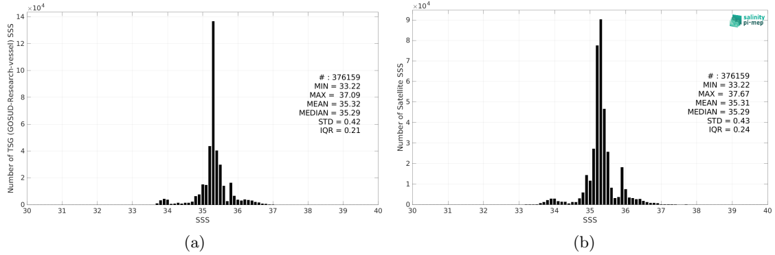
Figure 2: Histograms of SSS from TSG (GOSUD-Research-vessel) (a) and CCI SSS L4 Merged-OI v4.4 - 7-day running (ESA) (b) considering all match-up pairs per bins of 0.1 over the Indian Ocean Pi-MEP region and for the full satellite product period.
