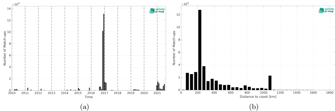
Figure 1: Number of match-ups between TSG (GOSUD-Research-vessel) and CCI SSS L4 Merged-OI v4.4 - 7-day running (ESA) SSS as a function of time (a) and as function of the distance to coast (b) over the Indian Ocean Pi-MEP region and for the full satellite product period.
