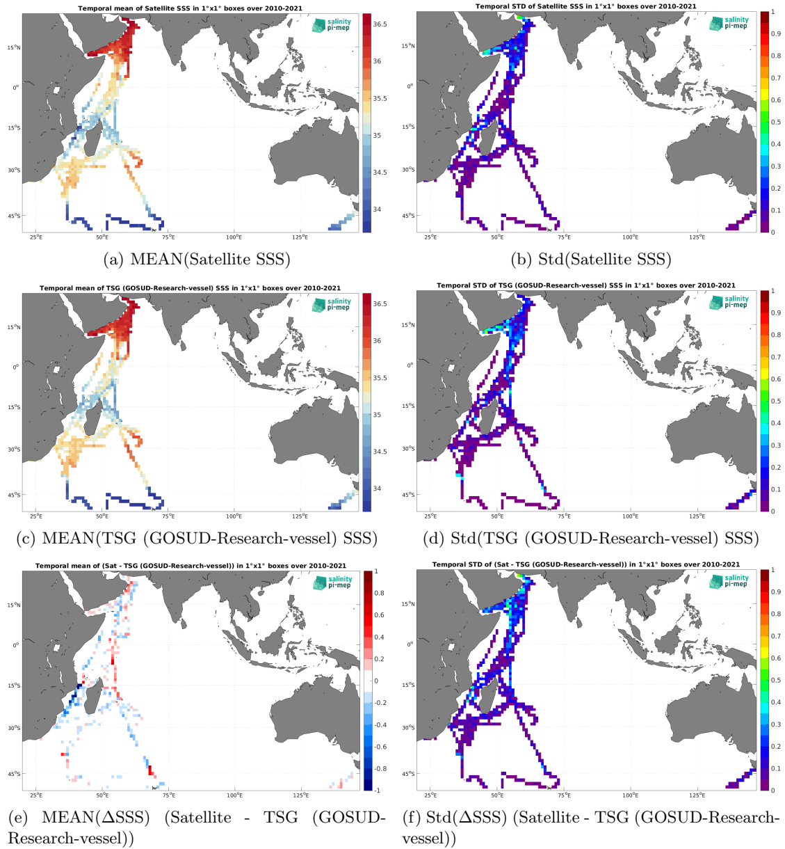
Figure 6: Temporal mean (left) and Std (right) of SSS from CCI SSS L4 Merged-OI v4.4 - 7-day running (ESA) (top), TSG (GOSUD-Research-vessel) (middle), and of \Delta SSS (Satellite - TSG (GOSUD-Research-vessel)). Only match-up pairs are used to generate these maps.
