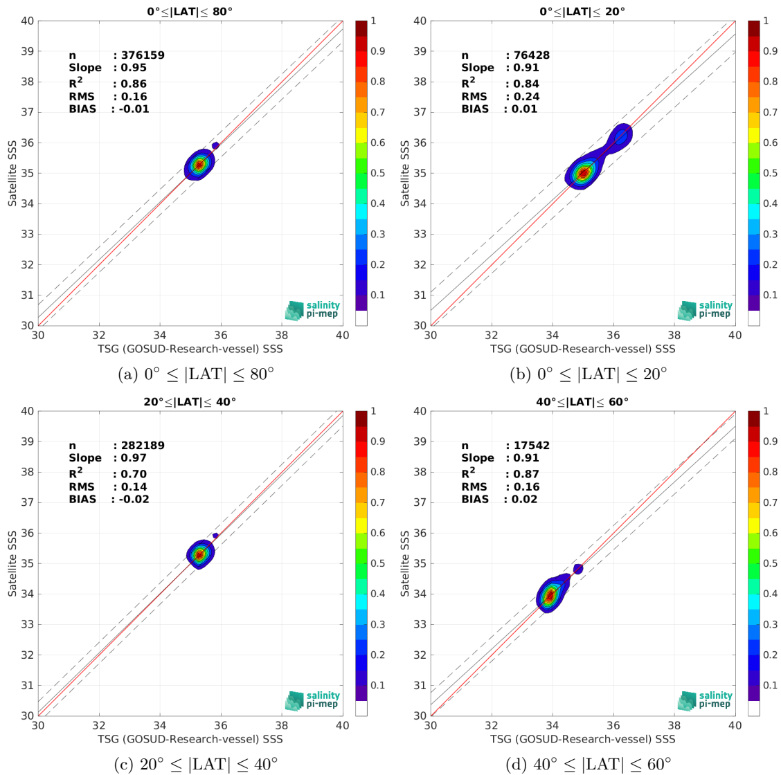
Figure 9: Contour maps of the concentration of CCI SSS L4 Merged-OI v4.4 - 7-day running (ESA) SSS (y-axis) versus TSG (GOSUD-Research-vessel) SSS (x-axis) at match-up pairs for different latitude bands. For each plot, the red line shows x=y . The black thin and dashed lines indicate a linear fit through the data cloud and the \pm 95\% confidence levels, respectively. The number match-up pairs n , the slope and R^2 coefficient of the linear fit, the root mean square (RMS) and the mean bias between satellite and in situ data are indicated for each latitude band in each plots.
