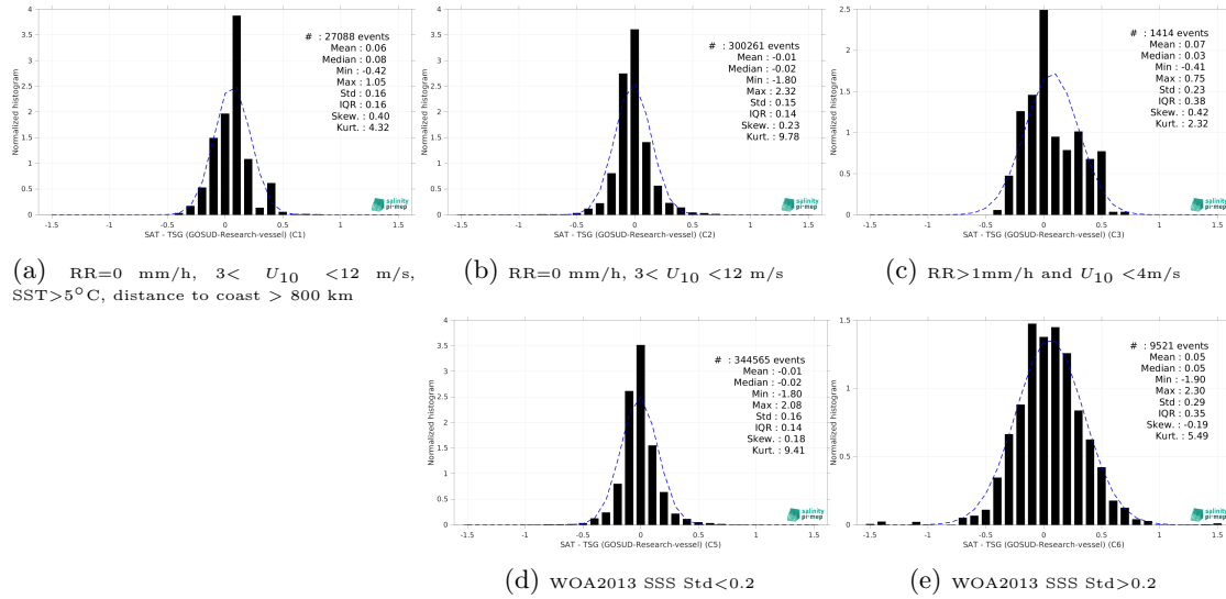
Figure 13: Normalized histogram of \Delta SSS (CCI SSS L4 Merged-OI v4.4 - 7-day running (ESA) - TSG (GOSUD-Research-vessel)) for 5 different subdatasets corresponding to: RR=0 mm/h, 3 < U_{10} < 12 m/s, SST>5°C, distance to coast > 800 km (a), RR=0 mm/h, 3 < U_{10} < 12 m/s (b), RR>1mm/h and U_{10} < 4 m/s (c), WOA2013 SSS Std<0.2 (d), WOA2013 SSS Std>0.2 (e).
