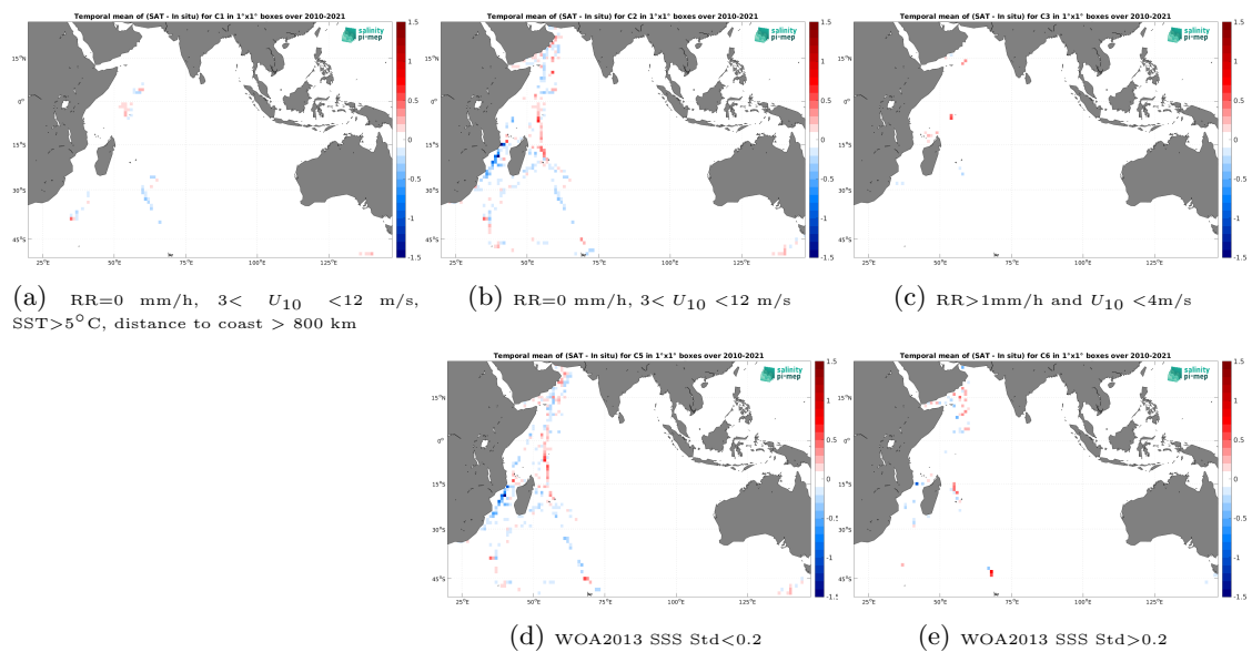
Figure 12: Temporal mean gridded over spatial boxes of size 1^\circ \times 1^\circ of \Delta SSS (CCI SSS L4 Merged-OI v4.4 - 7-day running (ESA) - TSG (GOSUD-Research-vessel)) for 5 different subdatasets corresponding to:RR=0 mm/h, 3 < U_{10} < 12 m/s, SST >5^\circ C, distance to coast > 800 km (a), RR=0 mm/h, 3 < U_{10} < 12 m/s (b), RR >1 mm/h and U_{10} < 4 m/s (c), WOA2013 SSS Std <0.2 (d), WOA2013 SSS Std >0.2 (e).
