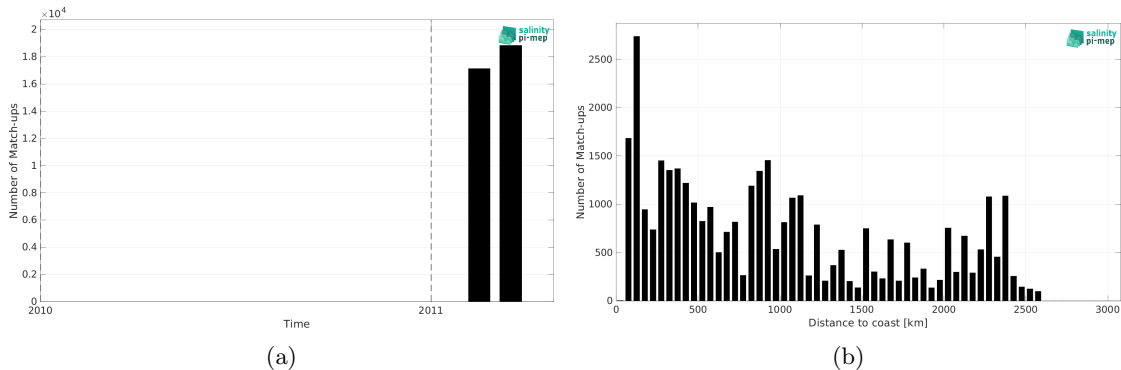
Figure 1: Number of match-ups between TSG (CSIC-UTM) and CCI SSS L4 Merged-OI v4.4 - 7-day running (ESA) SSS as a function of time (a) and as function of the distance to coast (b) over the Indian Ocean Pi-MEP region and for the full satellite product period.
