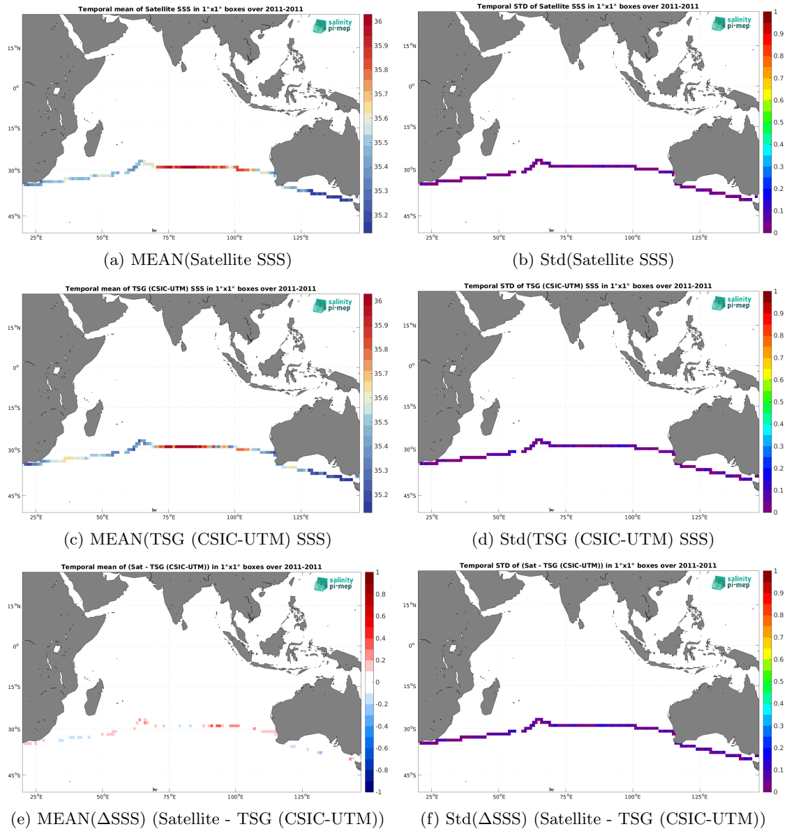
Figure 6: Temporal mean (left) and Std (right) of SSS from CCI SSS L4 Merged-OI v4.4 - 7-day running (ESA) (top), TSG (CSIC-UTM) (middle), and of \Delta SSS (Satellite - TSG (CSIC-UTM)). Only match-up pairs are used to generate these maps.
