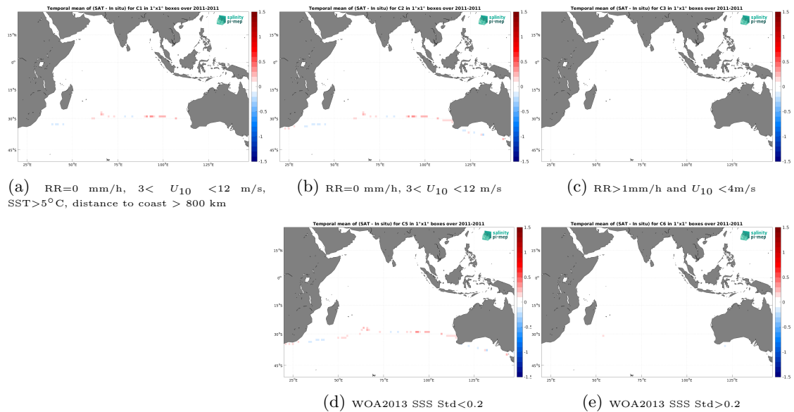
Figure 12: Temporal mean gridded over spatial boxes of size 1^\circ \times 1^\circ of \Delta SSS (CCI SSS L4 Merged-OI v4.4 - 7-day running (ESA) - TSG (CSIC-UTM)) for 5 different subdatasets corresponding to:RR=0 mm/h, 3 < U_{10} < 12 m/s, SST >5^\circ\text{C} , distance to coast > 800 km (a), RR=0 mm/h, 3 < U_{10} < 12 m/s (b), RR >1 mm/h and U_{10} < 4 m/s (c), WOA2013 SSS Std <0.2 (d), WOA2013 SSS Std >0.2 (e).
