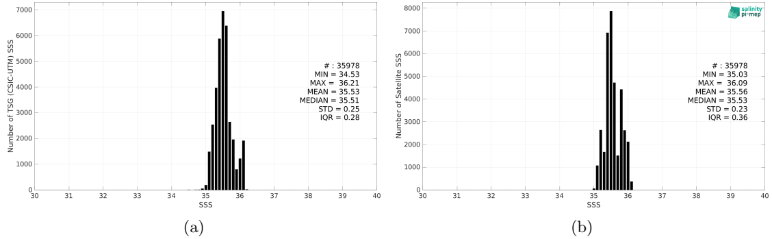
Figure 2: Histograms of SSS from TSG (CSIC-UTM) (a) and CCI SSS L4 Merged-OI v4.4 - 7-day running (ESA) (b) considering all match-up pairs per bins of 0.1 over the Indian Ocean Pi-MEP region and for the full satellite product period.
