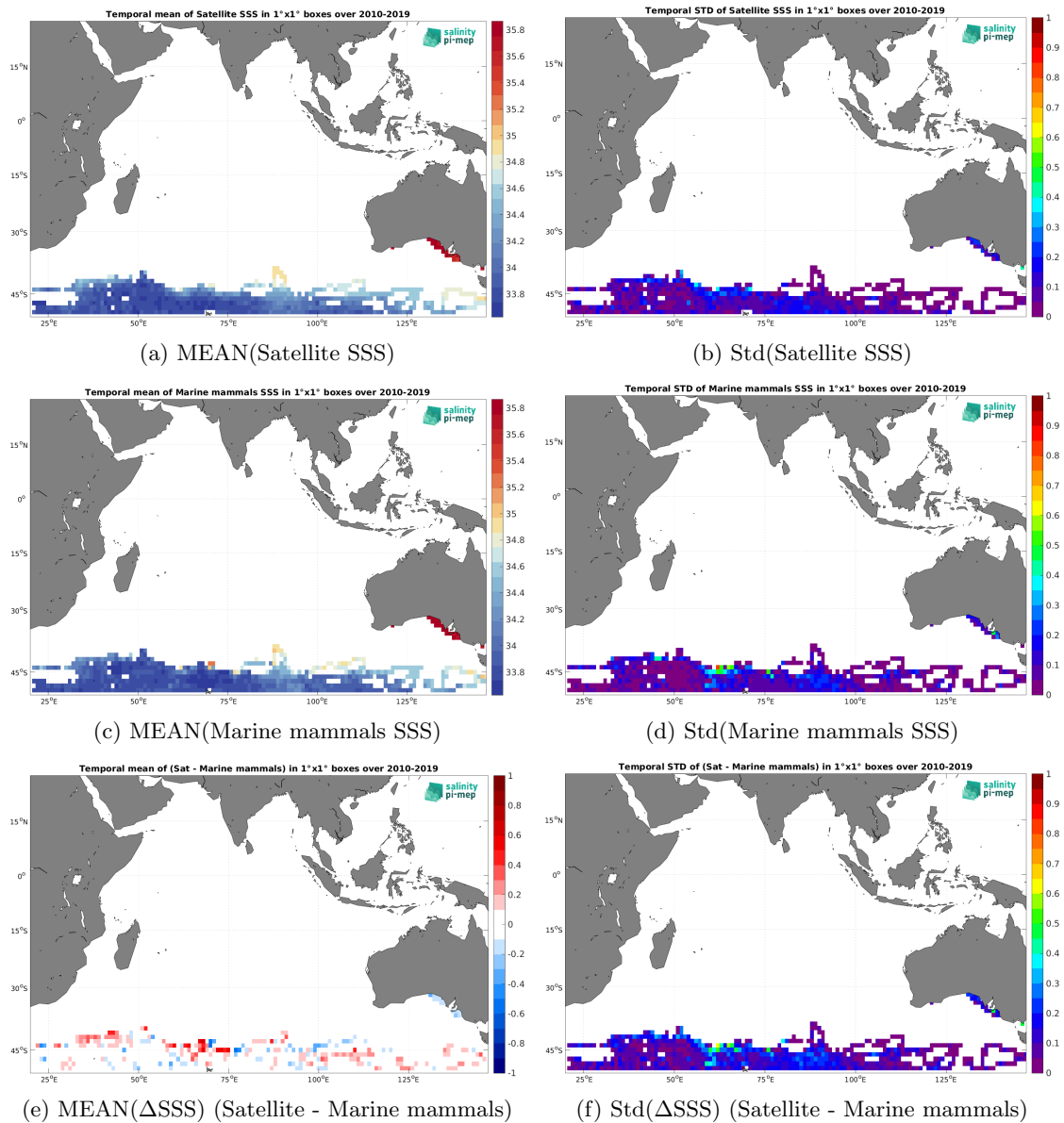
Figure 6: Temporal mean (left) and Std (right) of SSS from CCI SSS L4 Merged-OI v4.4 - 7-day running (ESA) (top), Marine mammals (middle), and of \Delta SSS (Satellite - Marine mammals). Only match-up pairs are used to generate these maps.
