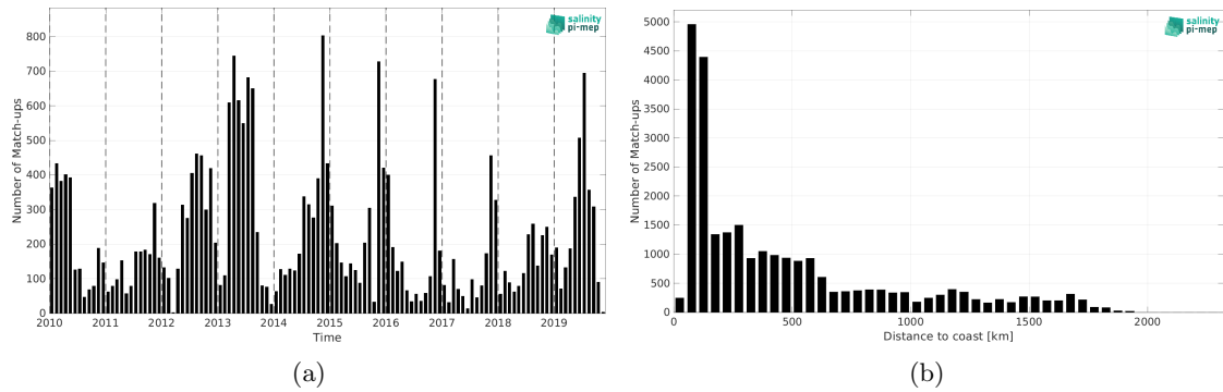
Figure 1: Number of match-ups between Marine mammals and CCI SSS L4 Merged-OI v4.4 - 7-day running (ESA) SSS as a function of time (a) and as function of the distance to coast (b) over the Indian Ocean Pi-MEP region and for the full satellite product period.
