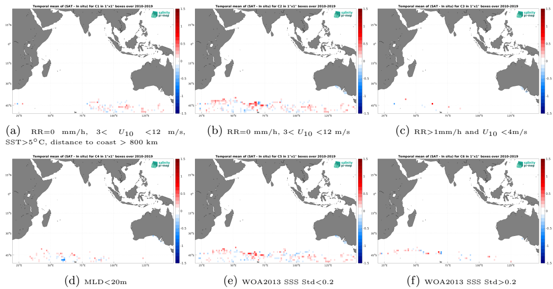
Figure 12: Temporal mean gridded over spatial boxes of size 1^\circ \times 1^\circ of \Delta SSS (CCI SSS L4 Merged-OI v4.4 - 7-day running (ESA) - Marine mammals) for 6 different subdatasets corresponding to:RR=0 mm/h, 3 < U_{10} < 12 m/s, SST >5^\circ C, distance to coast > 800 km (a), RR=0 mm/h, 3 < U_{10} < 12 m/s (b), RR >1 mm/h and U_{10} < 4 m/s (c),MLD <20 m (d),WOA2013 SSS Std <0.2 (e),WOA2013 SSS Std >0.2 (f).
