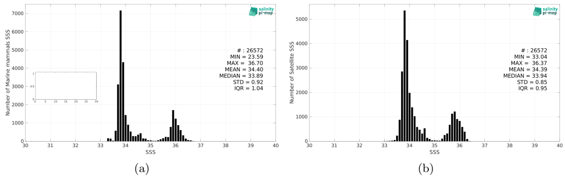
Figure 2: Histograms of SSS from Marine mammals (a) and CCI SSS L4 Merged-OI v4.4 - 7-day running (ESA) (b) considering all match-up pairs per bins of 0.1 over the Indian Ocean Pi-MEP region and for the full satellite product period.
