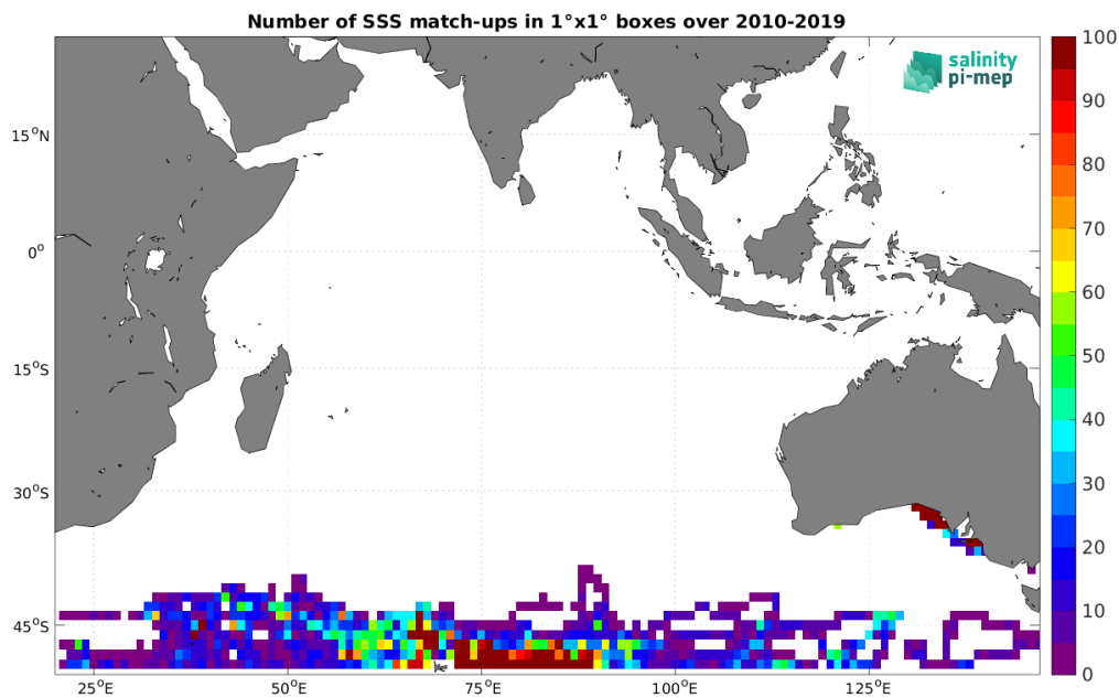
Figure 4: Number of SSS match-ups between Marine mammals SSS and the CCI SSS L4 Merged-OI v4.4 - 7-day running (ESA) SSS product for the Indian Ocean Pi-MEP region over 1^\circ \times 1^\circ boxes and for the full satellite product period.
