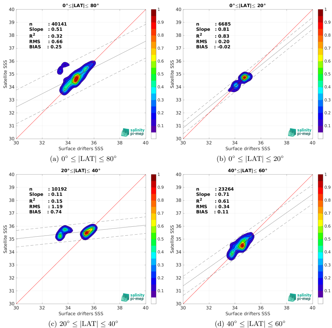
Figure 8: Contour maps of the concentration of CCI SSS L4 Merged-OI v4.4 - 7-day running (ESA) SSS (y-axis) versus Surface drifters SSS (x-axis) at match-up pairs for different latitude bands. For each plot, the red line shows x=y . The black thin and dashed lines indicate a linear fit through the data cloud and the \pm 95\% confidence levels, respectively. The number match-up pairs n , the slope and R^2 coefficient of the linear fit, the root mean square (RMS) and the mean bias between satellite and in situ data are indicated for each latitude band in each plots.
