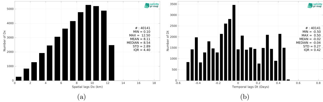
Figure 4: Histograms of the spatial (a) and temporal (b) lags between the location/time of the Surface drifters measurement and the date of the corresponding CCI SSS L4 Merged-OI v4.4 - 7-day running (ESA) SSS pixel.
