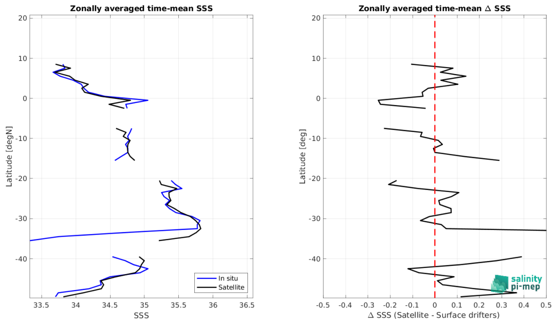
Figure 7: Left panel: Zonal mean SSS from CCI SSS L4 Merged-OI v4.4 - 7-day running (ESA) satellite product (black) and from Surface drifters (blue). Right panel: Zonal mean of \Delta SSS (Satellite - Surface drifters) for all the collected Pi-MEP match-up pairs estimated over the full satellite product period.
