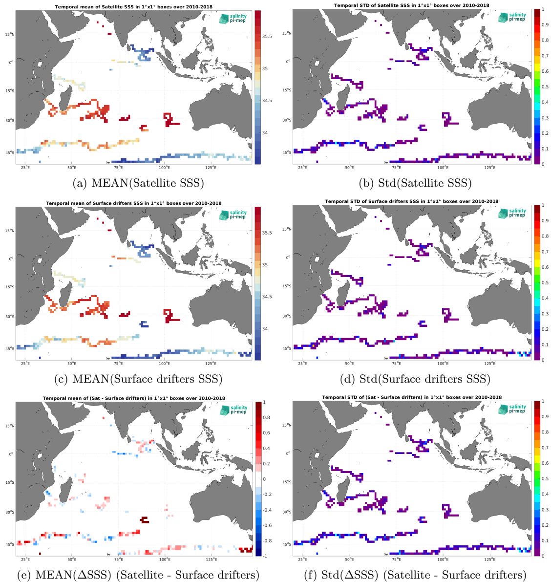
Figure 5: Temporal mean (left) and Std (right) of SSS from CCI SSS L4 Merged-OI v4.4 - 7-day running (ESA) (top), Surface drifters (middle), and of \Delta SSS (Satellite - Surface drifters). Only match-up pairs are used to generate these maps.
