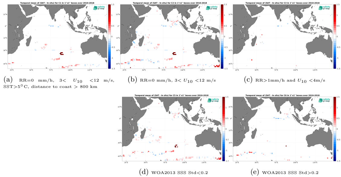
Figure 11: Temporal mean gridded over spatial boxes of size 1^\circ \times 1^\circ of \Delta\text{SSS} (CCI SSS L4 Merged-OI v4.4 - 7-day running (ESA) - Surface drifters) for 5 different subdatasets corresponding to:RR=0 mm/h, 3 < U_{10} < 12 m/s, SST >5^\circ\text{C} , distance to coast > 800 km (a), RR=0 mm/h, 3 < U_{10} < 12 m/s (b), RR >1 mm/h and U_{10} < 4 m/s (c), WOA2013 SSS Std <0.2 (d), WOA2013 SSS Std >0.2 (e).
