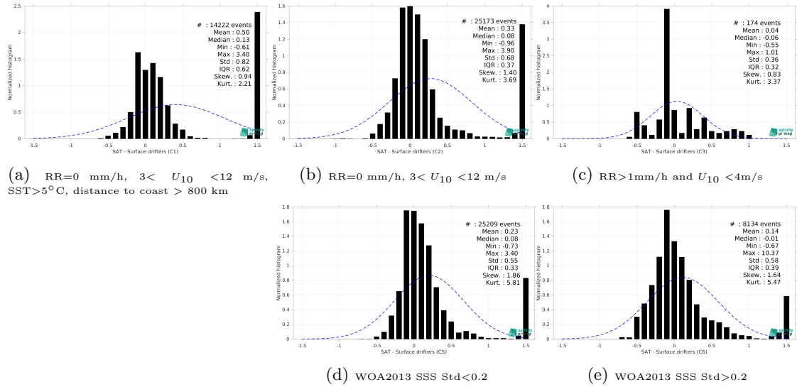
Figure 12: Normalized histogram of \Delta SSS (CCI SSS L4 Merged-OI v4.4 - 7-day running (ESA) - Surface drifters) for 5 different subdatasets corresponding to: RR=0 mm/h, 3 < U_{10} < 12 m/s, SST > 5°C, distance to coast > 800 km (a), RR=0 mm/h, 3 < U_{10} < 12 m/s (b), RR > 1mm/h and U_{10} < 4 m/s (c), WOA2013 SSS Std < 0.2 (d), WOA2013 SSS Std > 0.2 (e).
