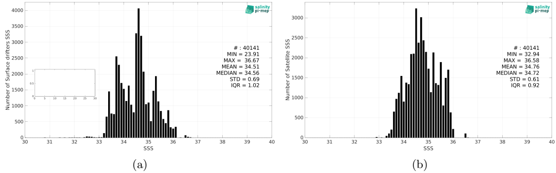
Figure 2: Histograms of SSS from Surface drifters (a) and CCI SSS L4 Merged-OI v4.4 - 7-day running (ESA) (b) considering all match-up pairs per bins of 0.1 over the Indian Ocean Pi-MEP region and for the full satellite product period.
