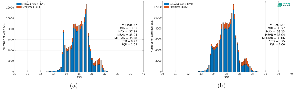
Figure 2: Histograms of SSS from Argo (a) and CCI SSS L4 Merged-OI v4.4 - 7-day running (ESA) (b) considering all match-up pairs per bins of 0.1 over the Indian Ocean Pi-MEP region and for the full satellite product period.
