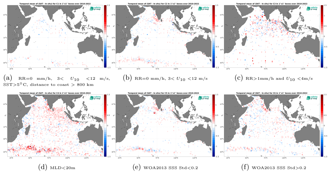
Figure 12: Temporal mean gridded over spatial boxes of size 1^\circ \times 1^\circ of \Delta SSS (CCI SSS L4 Merged-OI v4.4 - 7-day running (ESA) - Argo) for 6 different subdatasets corresponding to:RR=0 mm/h, 3 < U_{10} < 12 m/s, SST >5^\circ C, distance to coast > 800 km (a), RR=0 mm/h, 3 < U_{10} < 12 m/s (b), RR >1 mm/h and U_{10} < 4 m/s (c),MLD <20 m (d),WOA2013 SSS Std <0.2 (e),WOA2013 SSS Std >0.2 (f).
