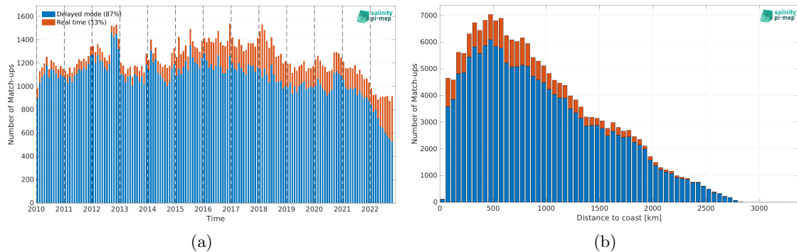
Figure 1: Number of match-ups between Argo and CCI SSS L4 Merged-OI v4.4 - 7-day running (ESA) SSS as a function of time (a) and as function of the distance to coast (b) over the Indian Ocean Pi-MEP region and for the full satellite product period.
