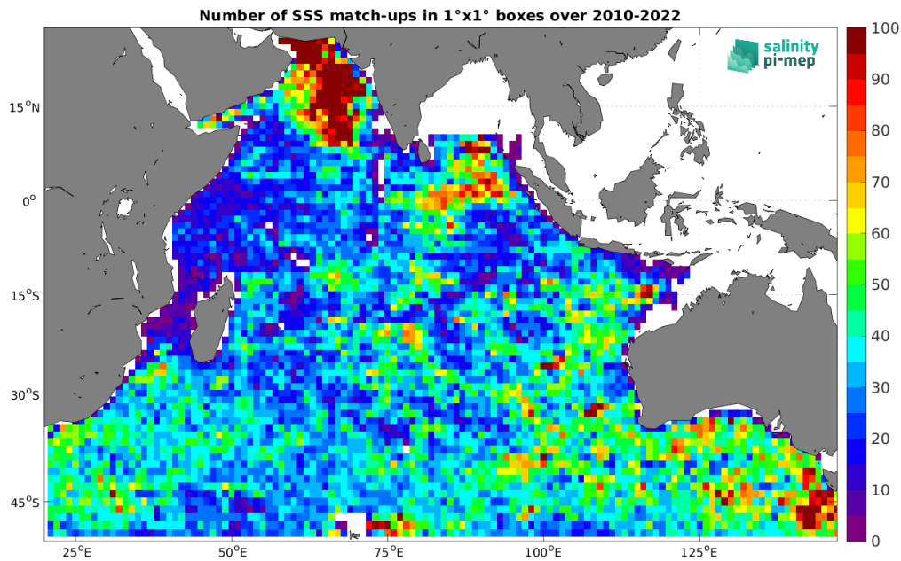
Figure 4: Number of SSS match-ups between Argo SSS and the CCI SSS L4 Merged-OI v4.4 - 7-day running (ESA) SSS product for the Indian Ocean Pi-MEP region over 1^\circ \times 1^\circ boxes and for the full satellite product period.
