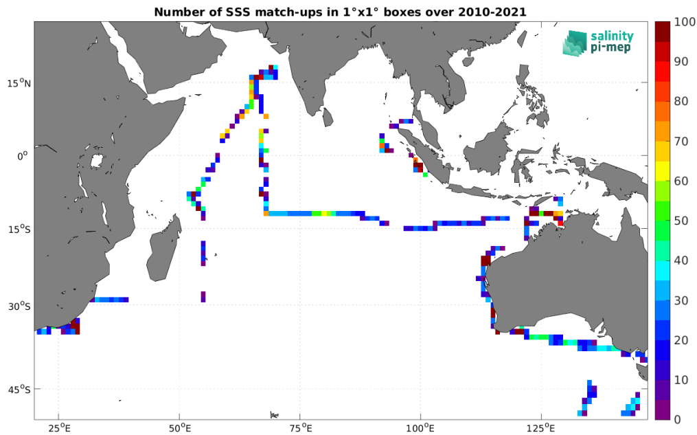
Figure 4: Number of SSS match-ups between TSG (SAMOS) SSS and the CCI SSS L4 Merged-OI v4.4 - 30-day running (ESA) SSS product for the Indian Ocean Pi-MEP region over 1^\circ \times 1^\circ boxes and for the full satellite product period.
