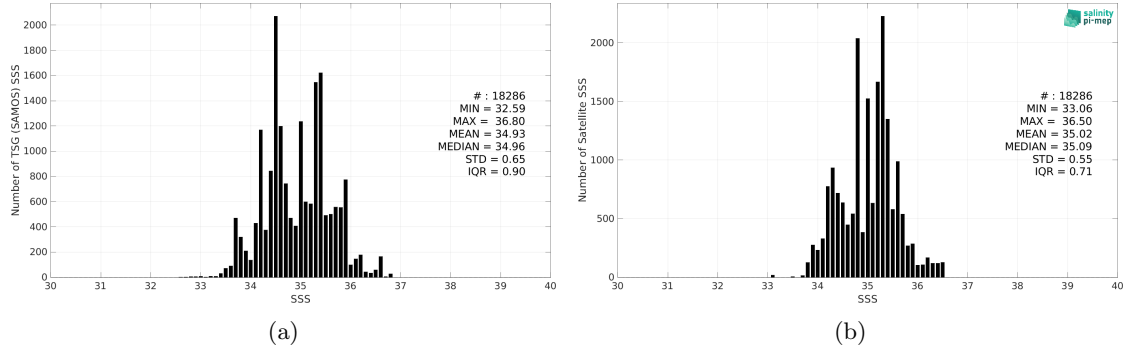
Figure 2: Histograms of SSS from TSG (SAMOS) (a) and CCI SSS L4 Merged-OI v4.4 - 30-day running (ESA) (b) considering all match-up pairs per bins of 0.1 over the Indian Ocean Pi-MEP region and for the full satellite product period.
