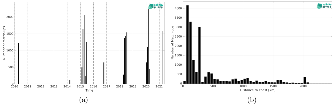
Figure 1: Number of match-ups between TSG (SAMOS) and CCI SSS L4 Merged-OI v4.4 - 30-day running (ESA) SSS as a function of time (a) and as function of the distance to coast (b) over the Indian Ocean Pi-MEP region and for the full satellite product period.
