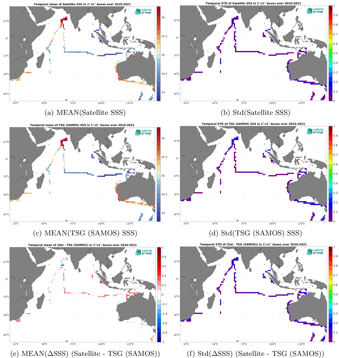
Figure 6: Temporal mean (left) and Std (right) of SSS from CCI SSS L4 Merged-OI v4.4 - 30-day running (ESA) (top), TSG (SAMOS) (middle), and of \Delta SSS (Satellite - TSG (SAMOS)). Only match-up pairs are used to generate these maps.
