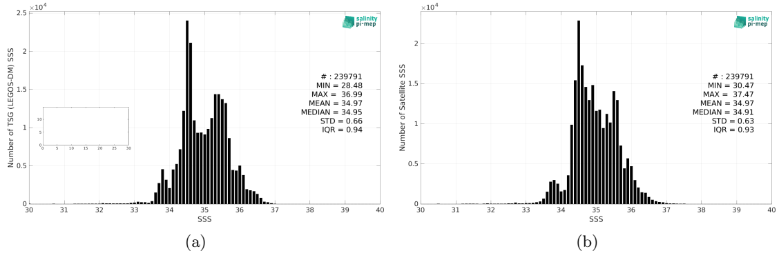
Figure 2: Histograms of SSS from TSG (LEGOS-DM) (a) and CCI SSS L4 Merged-OI v4.4 - 30-day running (ESA) (b) considering all match-up pairs per bins of 0.1 over the Indian Ocean Pi-MEP region and for the full satellite product period.
