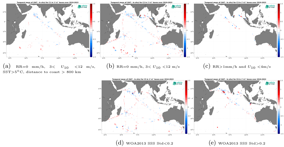
Figure 12: Temporal mean gridded over spatial boxes of size 1^\circ \times 1^\circ of \Delta SSS (CCI SSS L4 Merged-OI v4.4 - 30-day running (ESA) - TSG (LEGOS-DM)) for 5 different subdatasets corresponding to:RR=0 mm/h, 3 < U_{10} < 12 m/s, SST >5^\circ C, distance to coast > 800 km (a), RR=0 mm/h, 3 < U_{10} < 12 m/s (b), RR >1 mm/h and U_{10} < 4 m/s (c), WOA2013 SSS Std <0.2 (d), WOA2013 SSS Std >0.2 (e).
