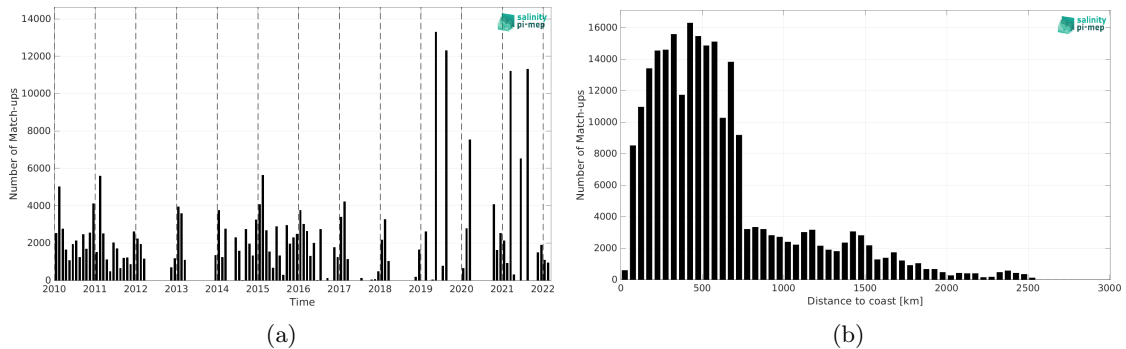
Figure 1: Number of match-ups between TSG (LEGOS-DM) and CCI SSS L4 Merged-OI v4.4 - 30-day running (ESA) SSS as a function of time (a) and as function of the distance to coast (b) over the Indian Ocean Pi-MEP region and for the full satellite product period.
