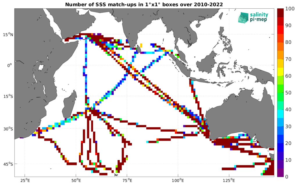
Figure 4: Number of SSS match-ups between TSG (LEGOS-DM) SSS and the CCI SSS L4 Merged-OI v4.4 - 30-day running (ESA) SSS product for the Indian Ocean Pi-MEP region over 1^\circ \times 1^\circ boxes and for the full satellite product period.
