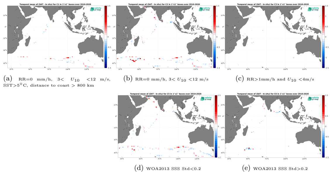
Figure 12: Temporal mean gridded over spatial boxes of size 1^\circ \times 1^\circ of \Delta\text{SSS} (CCI SSS L4 Merged-OI v4.4 - 30-day running (ESA) - TSG (GOSUD-Sailing-ship)) for 5 different subdatasets corresponding to:RR=0 mm/h, 3 < U_{10} < 12 m/s, SST >5^\circ\text{C} , distance to coast > 800 km (a), RR=0 mm/h, 3 < U_{10} < 12 m/s (b), RR >1 mm/h and U_{10} < 4 m/s (c), WOA2013 SSS Std <0.2 (d), WOA2013 SSS Std >0.2 (e).
