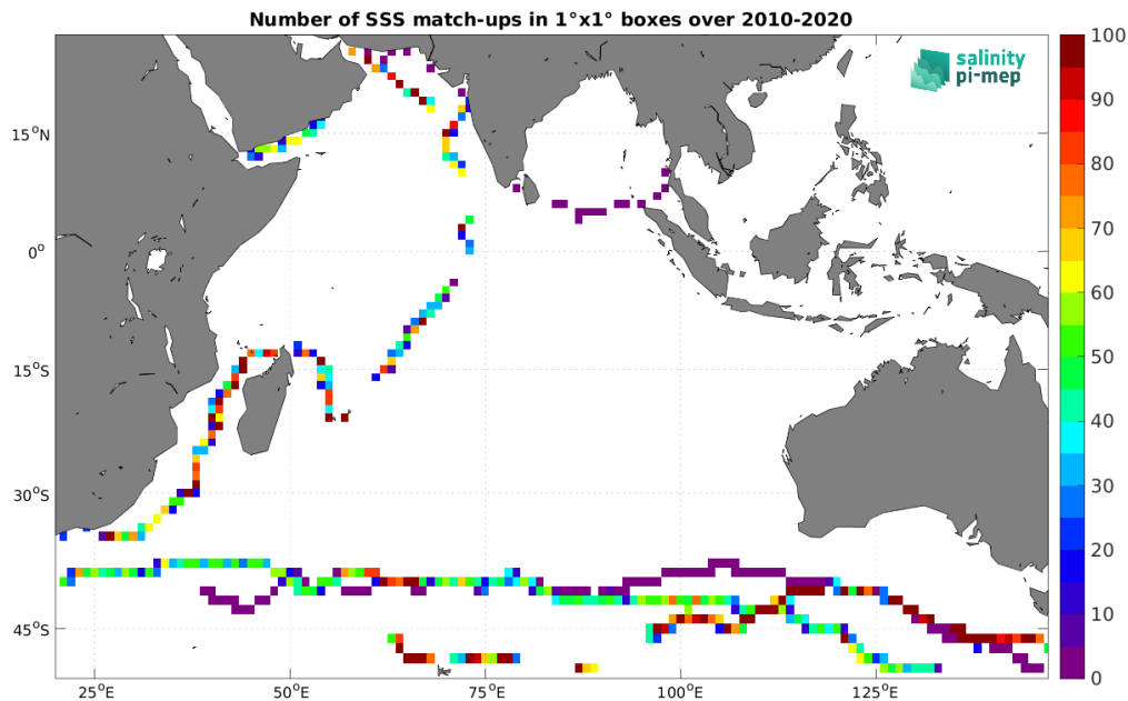
Figure 4: Number of SSS match-ups between TSG (GOSUD-Sailing-ship) SSS and the CCI SSS L4 Merged-OI v4.4 - 30-day running (ESA) SSS product for the Indian Ocean Pi-MEP region over 1^\circ \times 1^\circ boxes and for the full satellite product period.
