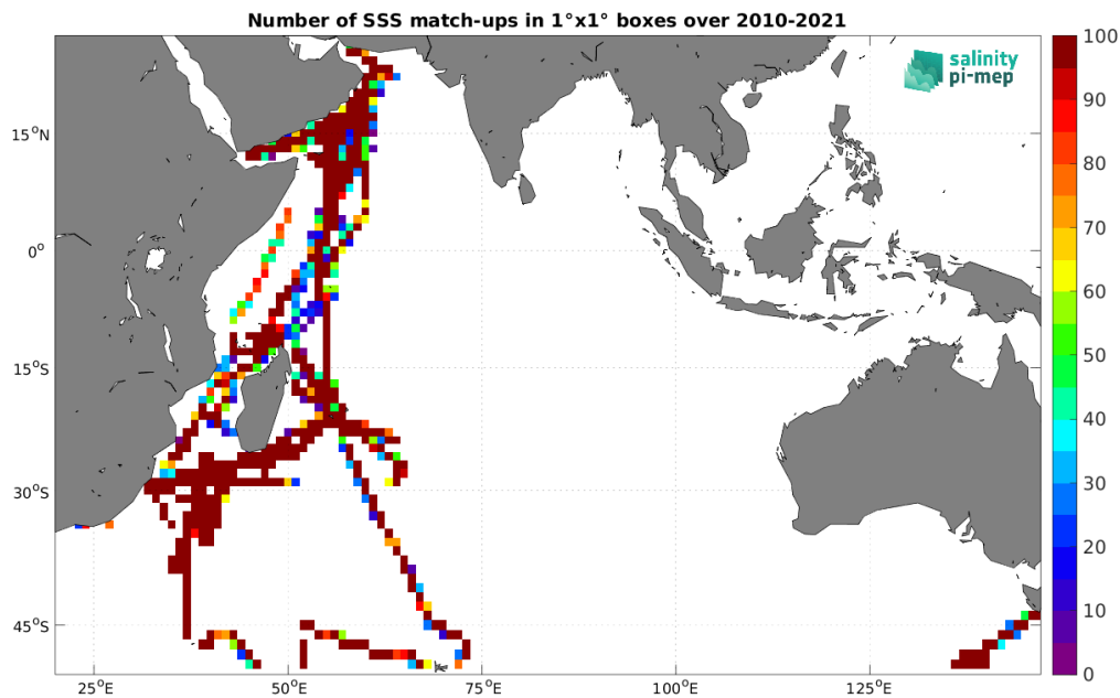
Figure 4: Number of SSS match-ups between TSG (GOSUD-Research-vessel) SSS and the CCI SSS L4 Merged-OI v4.4 - 30-day running (ESA) SSS product for the Indian Ocean Pi-MEP region over 1^\circ \times 1^\circ boxes and for the full satellite product period.
