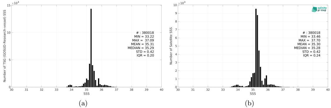
Figure 2: Histograms of SSS from TSG (GOSUD-Research-vessel) (a) and CCI SSS L4 Merged-OI v4.4 - 30-day running (ESA) (b) considering all match-up pairs per bins of 0.1 over the Indian Ocean Pi-MEP region and for the full satellite product period.
