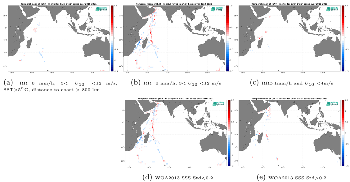
Figure 12: Temporal mean gridded over spatial boxes of size 1^\circ \times 1^\circ of \Delta SSS (CCI SSS L4 Merged-OI v4.4 - 30-day running (ESA) - TSG (GOSUD-Research-vessel)) for 5 different subdatasets corresponding to:RR=0 mm/h, 3 < U_{10} < 12 m/s, SST >5^\circ\text{C} , distance to coast > 800 km (a), RR=0 mm/h, 3 < U_{10} < 12 m/s (b), RR >1 mm/h and U_{10} < 4 m/s (c), WOA2013 SSS Std <0.2 (d), WOA2013 SSS Std >0.2 (e).
