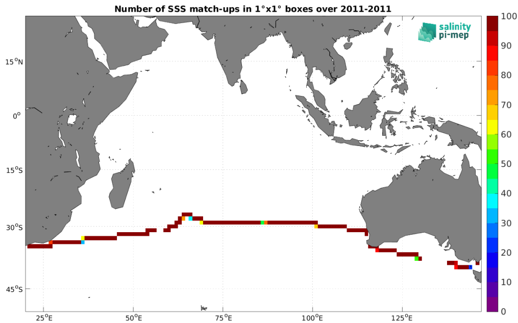
Figure 4: Number of SSS match-ups between TSG (CSIC-UTM) SSS and the CCI SSS L4 Merged-OI v4.4 - 30-day running (ESA) SSS product for the Indian Ocean Pi-MEP region over 1^\circ \times 1^\circ boxes and for the full satellite product period.
