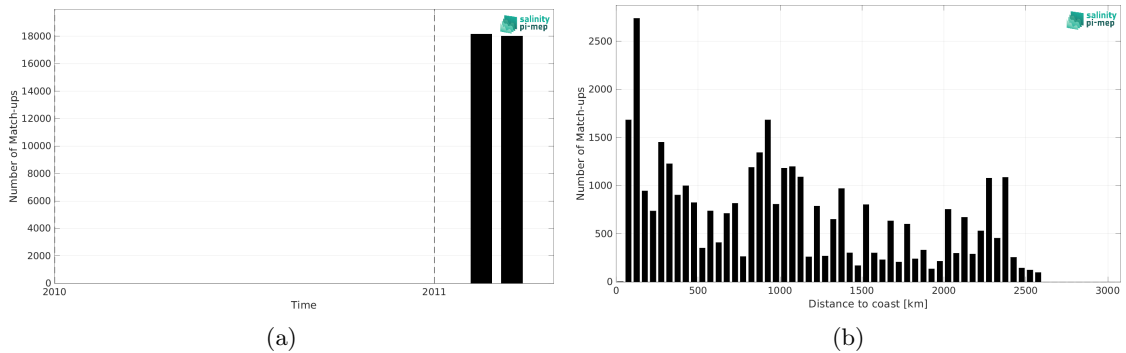
Figure 1: Number of match-ups between TSG (CSIC-UTM) and CCI SSS L4 Merged-OI v4.4 - 30-day running (ESA) SSS as a function of time (a) and as function of the distance to coast (b) over the Indian Ocean Pi-MEP region and for the full satellite product period.
