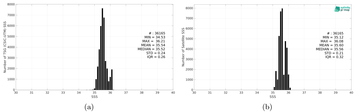
Figure 2: Histograms of SSS from TSG (CSIC-UTM) (a) and CCI SSS L4 Merged-OI v4.4 - 30-day running (ESA) (b) considering all match-up pairs per bins of 0.1 over the Indian Ocean Pi-MEP region and for the full satellite product period.
