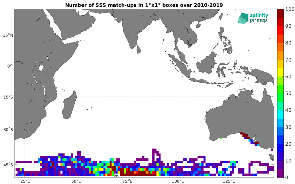
Figure 4: Number of SSS match-ups between Marine mammals SSS and the CCI SSS L4 Merged-OI v4.4 - 30-day running (ESA) SSS product for the Indian Ocean Pi-MEP region over 1^\circ \times 1^\circ boxes and for the full satellite product period.
