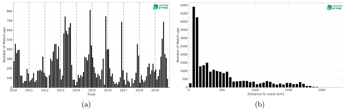
Figure 1: Number of match-ups between Marine mammals and CCI SSS L4 Merged-OI v4.4 - 30-day running (ESA) SSS as a function of time (a) and as function of the distance to coast (b) over the Indian Ocean Pi-MEP region and for the full satellite product period.
