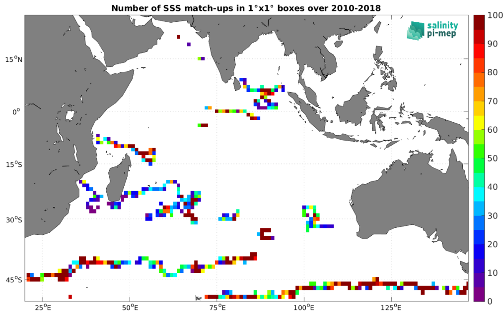
Figure 3: Number of SSS match-ups between Surface drifters SSS and the CCI SSS L4 Merged-OI v4.4 - 30-day running (ESA) SSS product for the Indian Ocean Pi-MEP region over 1^\circ \times 1^\circ boxes and for the full satellite product period.
