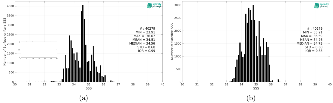
Figure 2: Histograms of SSS from Surface drifters (a) and CCI SSS L4 Merged-OI v4.4 - 30-day running (ESA) (b) considering all match-up pairs per bins of 0.1 over the Indian Ocean Pi-MEP region and for the full satellite product period.
