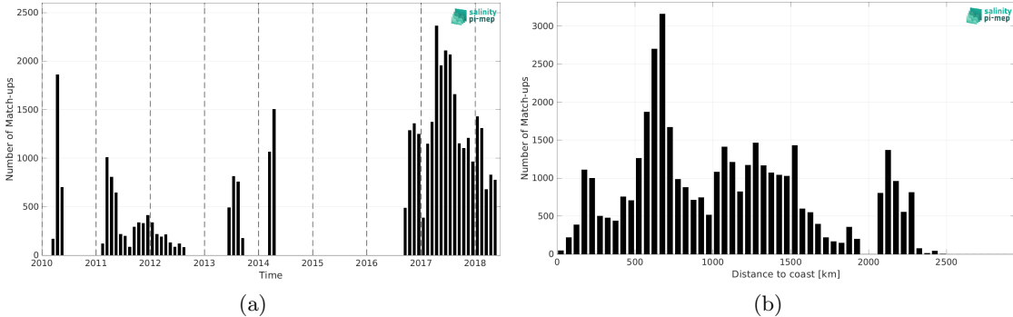
Figure 1: Number of match-ups between Surface drifters and CCI SSS L4 Merged-OI v4.4 - 30-day running (ESA) SSS as a function of time (a) and as function of the distance to coast (b) over the Indian Ocean Pi-MEP region and for the full satellite product period.
