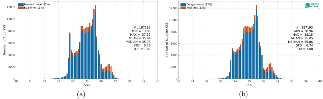
Figure 2: Histograms of SSS from Argo (a) and CCI SSS L4 Merged-OI v4.4 - 30-day running (ESA) (b) considering all match-up pairs per bins of 0.1 over the Indian Ocean Pi-MEP region and for the full satellite product period.
