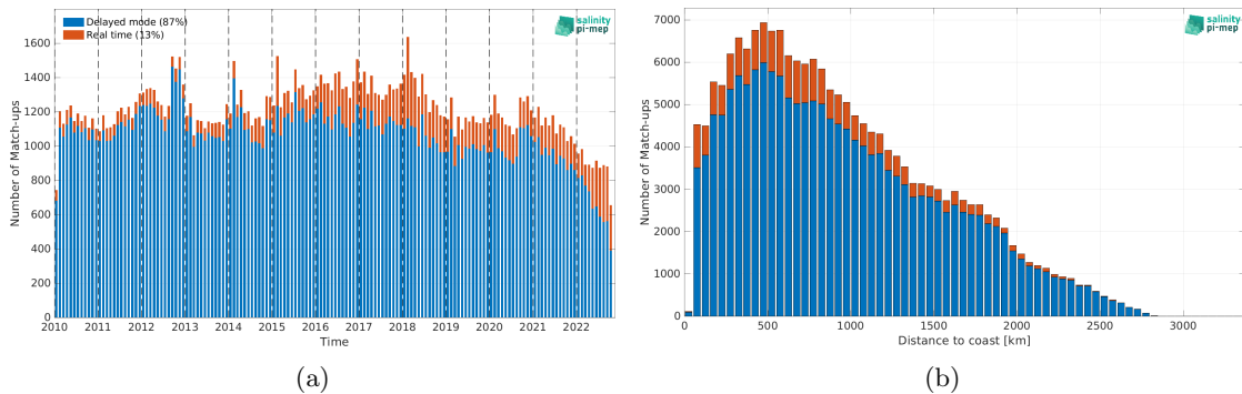
Figure 1: Number of match-ups between Argo and CCI SSS L4 Merged-OI v4.4 - 30-day running (ESA) SSS as a function of time (a) and as function of the distance to coast (b) over the Indian Ocean Pi-MEP region and for the full satellite product period.
