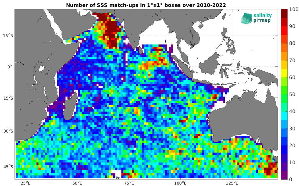
Figure 4: Number of SSS match-ups between Argo SSS and the CCI SSS L4 Merged-OI v4.4 - 30-day running (ESA) SSS product for the Indian Ocean Pi-MEP region over 1^\circ \times 1^\circ boxes and for the full satellite product period.
