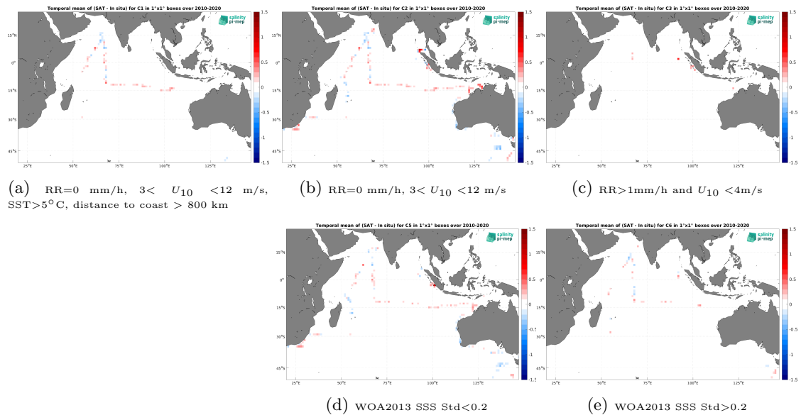
Figure 12: Temporal mean gridded over spatial boxes of size 1^\circ \times 1^\circ of \Delta\text{SSS} (CCI SSS L4 Merged-OI v3.2 - 7-day running (ESA) - TSG (SAMOS)) for 5 different subdatasets corresponding to:RR=0 mm/h, 3 < U_{10} < 12 m/s, SST >5^\circ\text{C} , distance to coast > 800 km (a), RR=0 mm/h, 3 < U_{10} < 12 m/s (b), RR >1 mm/h and U_{10} < 4 m/s (c), WOA2013 SSS Std <0.2 (d), WOA2013 SSS Std >0.2 (e).
