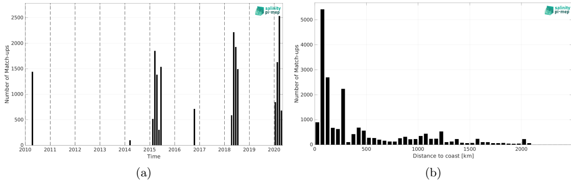
Figure 1: Number of match-ups between TSG (SAMOS) and CCI SSS L4 Merged-OI v3.2 - 7-day running (ESA) SSS as a function of time (a) and as function of the distance to coast (b) over the Indian Ocean Pi-MEP region and for the full satellite product period.
