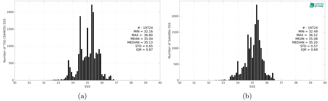
Figure 2: Histograms of SSS from TSG (SAMOS) (a) and CCI SSS L4 Merged-OI v3.2 - 7-day running (ESA) (b) considering all match-up pairs per bins of 0.1 over the Indian Ocean Pi-MEP region and for the full satellite product period.
