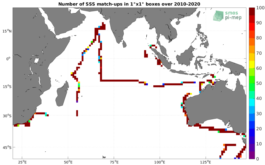
Figure 4: Number of SSS match-ups between TSG (SAMOS) SSS and the CCI SSS L4 Merged-OI v3.2 - 7-day running (ESA) SSS product for the Indian Ocean Pi-MEP region over 1^\circ \times 1^\circ boxes and for the full satellite product period.
