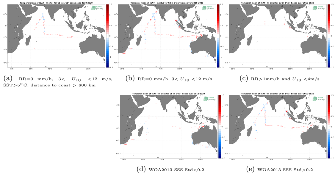
Figure 12: Temporal mean gridded over spatial boxes of size 1^\circ \times 1^\circ of \Delta SSS (CCI SSS L4 Merged-OI v3.2 - 7-day running (ESA) - TSG (SAMOS)) for 5 different subdatasets corresponding to:RR=0 mm/h, 3 < U_{10} < 12 m/s, SST >5^\circ\text{C} , distance to coast > 800 km (a), RR=0 mm/h, 3 < U_{10} < 12 m/s (b), RR >1\text{mm/h} and U_{10} < 4\text{m/s} (c), WOA2013 SSS Std <0.2 (d), WOA2013 SSS Std >0.2 (e).
