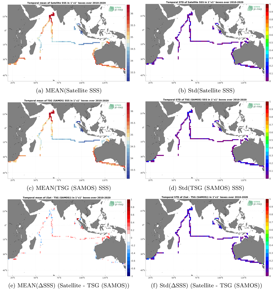
Figure 6: Temporal mean (left) and Std (right) of SSS from CCI SSS L4 Merged-OI v3.2 - 7-day running (ESA) (top), TSG (SAMOS) (middle), and of \Delta SSS (Satellite - TSG (SAMOS)). Only match-up pairs are used to generate these maps.
