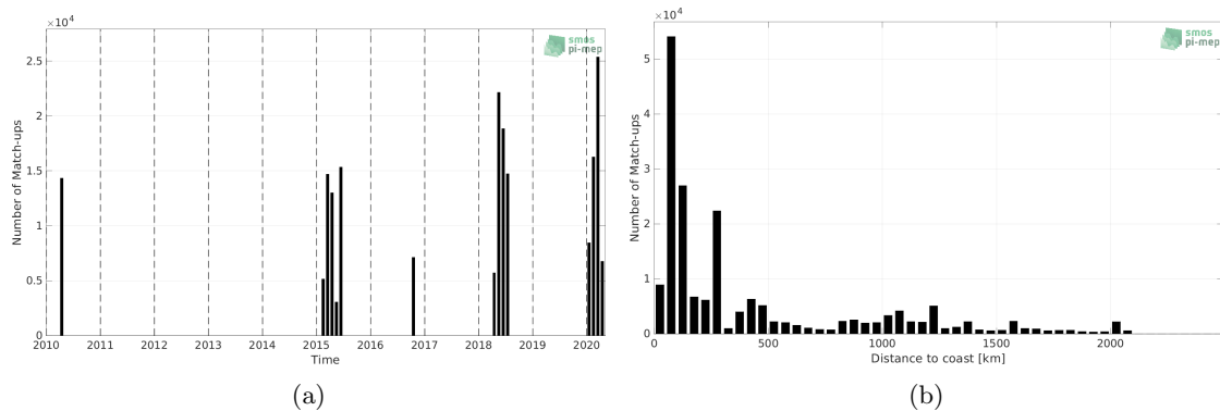
Figure 1: Number of match-ups between TSG (SAMOS) and CCI SSS L4 Merged-OI v3.2 - 7-day running (ESA) SSS as a function of time (a) and as function of the distance to coast (b) over the Indian Ocean Pi-MEP region and for the full satellite product period.
