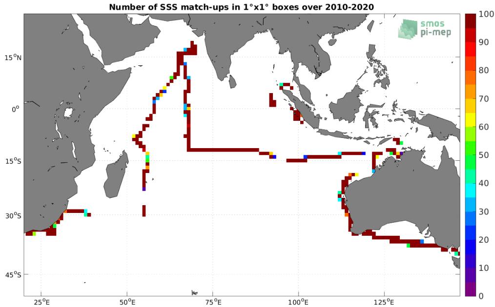
Figure 4: Number of SSS match-ups between TSG (SAMOS) SSS and the CCI SSS L4 Merged-OI v3.2 - 7-day running (ESA) SSS product for the Indian Ocean Pi-MEP region over 1^\circ \times 1^\circ boxes and for the full satellite product period.
