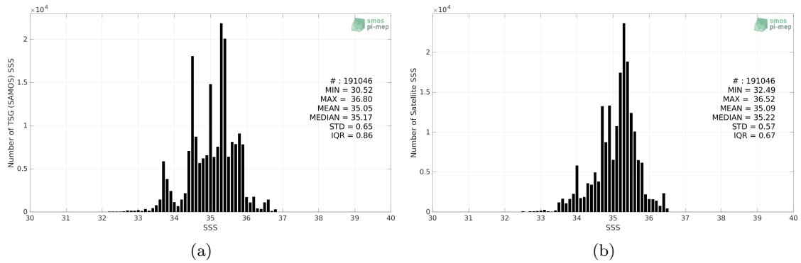
Figure 2: Histograms of SSS from TSG (SAMOS) (a) and CCI SSS L4 Merged-OI v3.2 - 7-day running (ESA) (b) considering all match-up pairs per bins of 0.1 over the Indian Ocean Pi-MEP region and for the full satellite product period.
