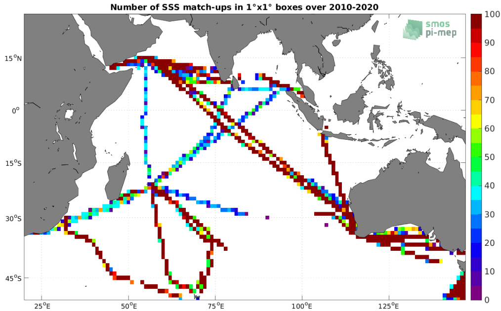
Figure 4: Number of SSS match-ups between TSG (LEGOS-DM) SSS and the CCI SSS L4 Merged-OI v3.2 - 7-day running (ESA) SSS product for the Indian Ocean Pi-MEP region over 1^\circ \times 1^\circ boxes and for the full satellite product period.
