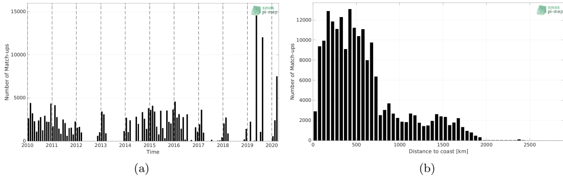
Figure 1: Number of match-ups between TSG (LEGOS-DM) and CCI SSS L4 Merged-OI v3.2 - 7-day running (ESA) SSS as a function of time (a) and as function of the distance to coast (b) over the Indian Ocean Pi-MEP region and for the full satellite product period.
