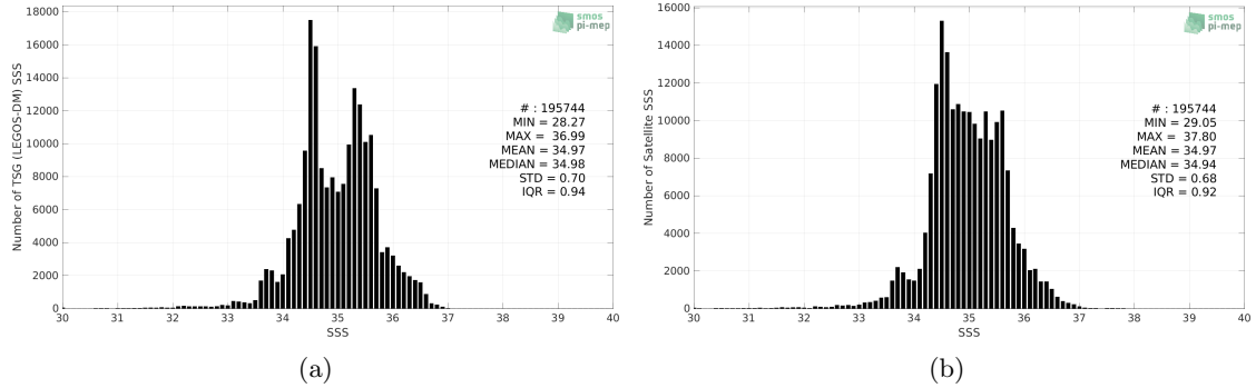
Figure 2: Histograms of SSS from TSG (LEGOS-DM) (a) and CCI SSS L4 Merged-OI v3.2 - 7-day running (ESA) (b) considering all match-up pairs per bins of 0.1 over the Indian Ocean Pi-MEP region and for the full satellite product period.
