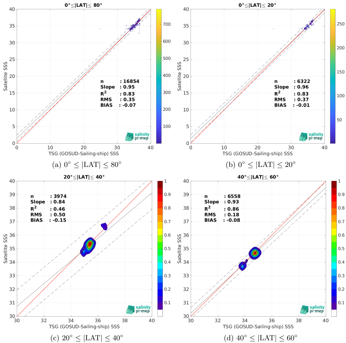
Figure 9: Contour maps of the concentration of CCI SSS L4 Merged-OI v3.2 - 7-day running (ESA) SSS (y-axis) versus TSG (GOSUD-Sailing-ship) SSS (x-axis) at match-up pairs for different latitude bands. For each plot, the red line shows x=y . The black thin and dashed lines indicate a linear fit through the data cloud and the \pm 95\% confidence levels, respectively. The number match-up pairs n , the slope and R^2 coefficient of the linear fit, the root mean square (RMS) and the mean bias between satellite and in situ data are indicated for each latitude band in each plots.
