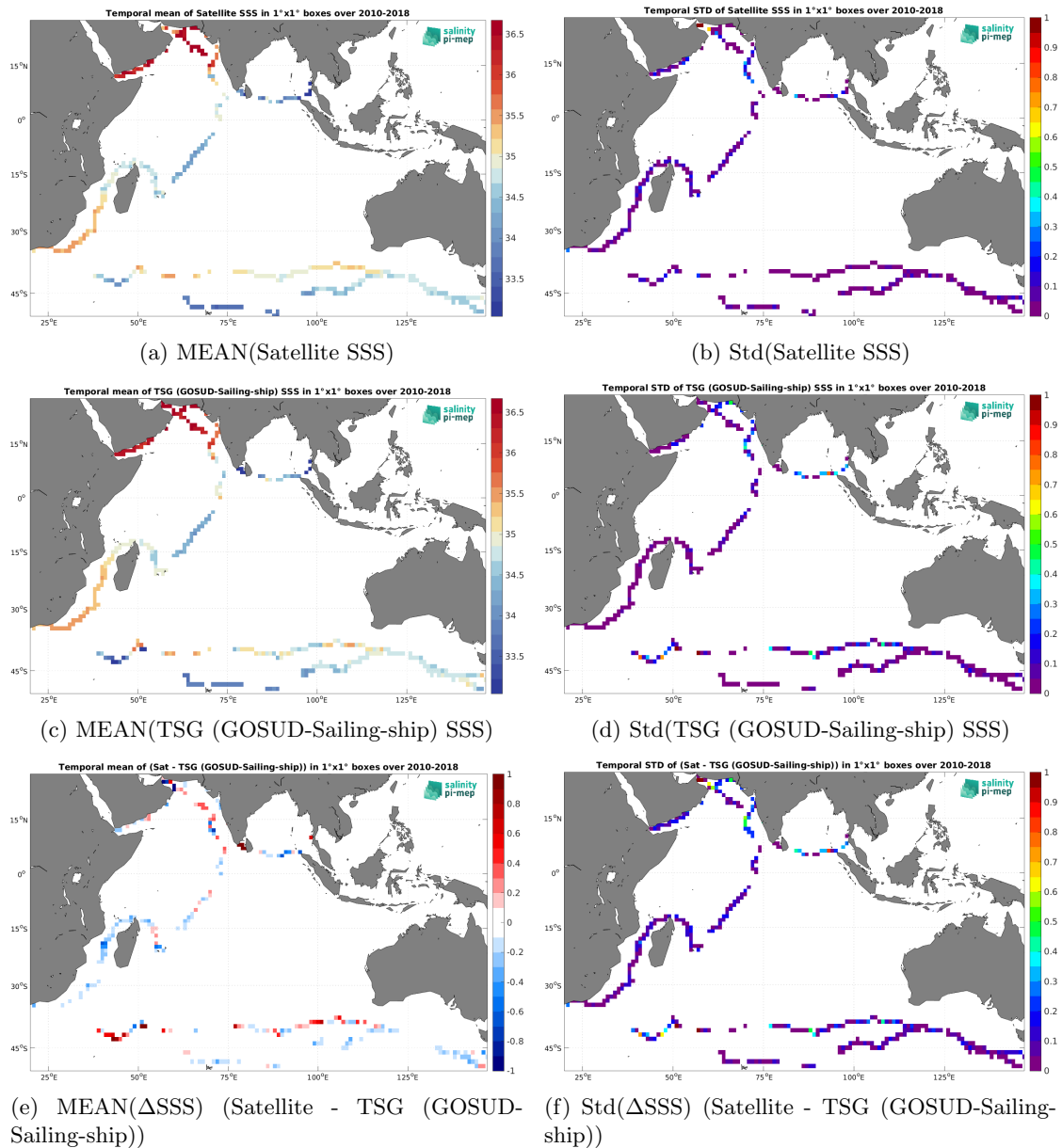
Figure 6: Temporal mean (left) and Std (right) of SSS from CCI SSS L4 Merged-OI v3.2 - 7-day running (ESA) (top), TSG (GOSUD-Sailing-ship) (middle), and of \Delta SSS (Satellite - TSG (GOSUD-Sailing-ship)). Only match-up pairs are used to generate these maps.
