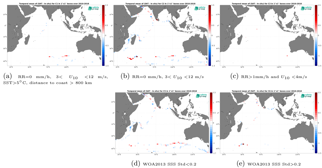
Figure 12: Temporal mean gridded over spatial boxes of size 1^\circ \times 1^\circ of \Delta SSS (CCI SSS L4 Merged-OI v3.2 - 7-day running (ESA) - TSG (GOSUD-Sailing-ship)) for 5 different subdatasets corresponding to:RR=0 mm/h, 3 < U_{10} < 12 m/s, SST >5^\circ\text{C} , distance to coast > 800 km (a), RR=0 mm/h, 3 < U_{10} < 12 m/s (b), RR >1 mm/h and U_{10} < 4 m/s (c), WOA2013 SSS Std <0.2 (d), WOA2013 SSS Std >0.2 (e).
