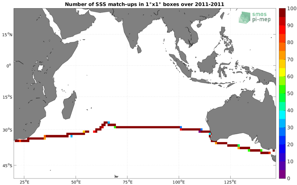
Figure 4: Number of SSS match-ups between TSG (CSIC-UTM) SSS and the CCI SSS L4 Merged-OI v3.2 - 7-day running (ESA) SSS product for the Indian Ocean Pi-MEP region over 1^\circ \times 1^\circ boxes and for the full satellite product period.
