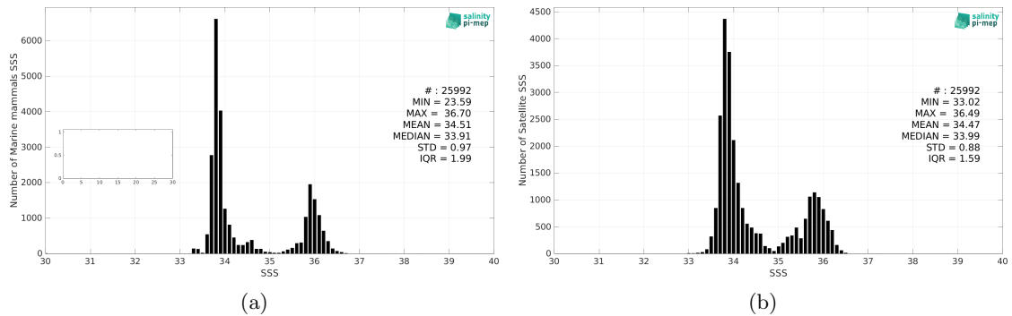
Figure 2: Histograms of SSS from Marine mammals (a) and CCI SSS L4 Merged-OI v3.2 - 7-day running (ESA) (b) considering all match-up pairs per bins of 0.1 over the Indian Ocean Pi-MEP region and for the full satellite product period.
