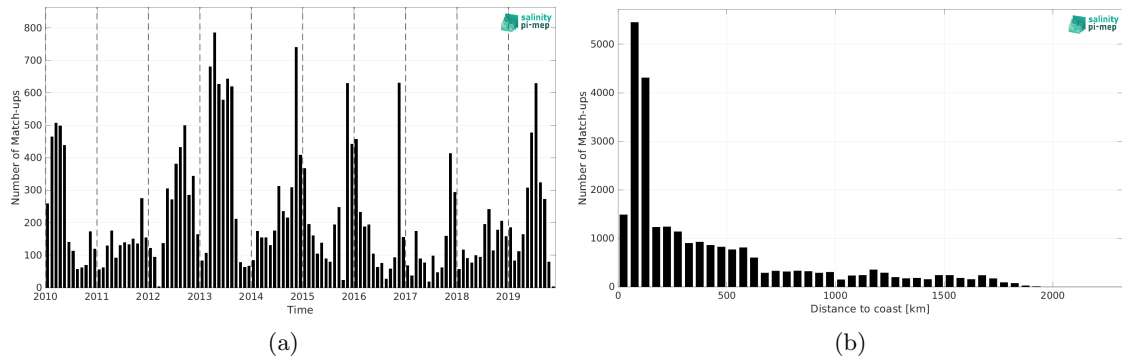
Figure 1: Number of match-ups between Marine mammals and CCI SSS L4 Merged-OI v3.2 - 7-day running (ESA) SSS as a function of time (a) and as function of the distance to coast (b) over the Indian Ocean Pi-MEP region and for the full satellite product period.
