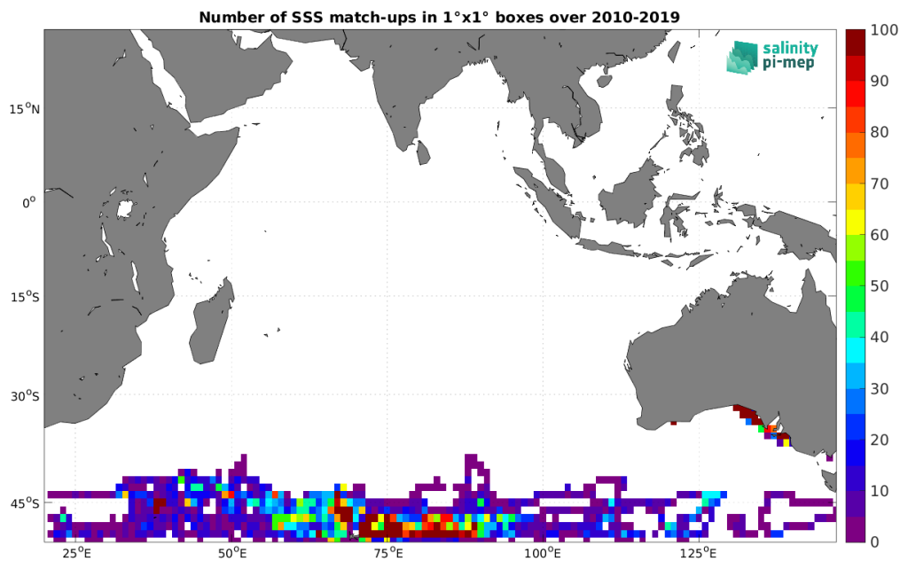
Figure 4: Number of SSS match-ups between Marine mammals SSS and the CCI SSS L4 Merged-OI v3.2 - 7-day running (ESA) SSS product for the Indian Ocean Pi-MEP region over 1^\circ \times 1^\circ boxes and for the full satellite product period.
