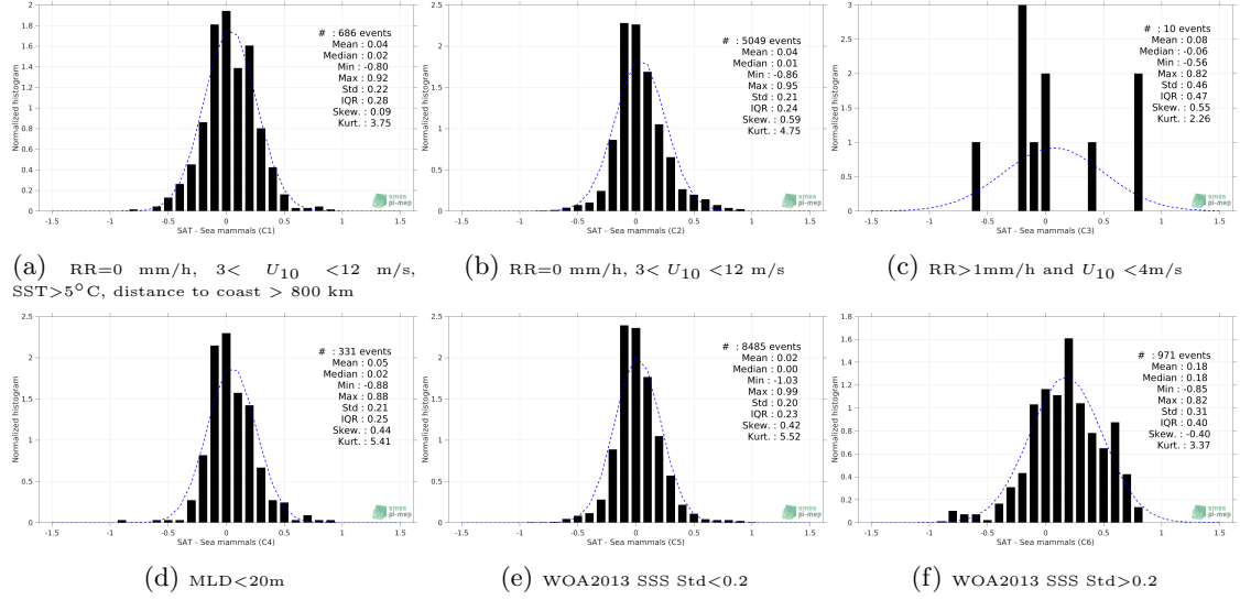
Figure 13: Normalized histogram of \Delta SSS (CCI SSS L4 Merged-OI v3.2 - 7-day running (ESA) - Sea mammals) for 6 different subdatasets corresponding to: RR=0 mm/h, 3 < U_{10} < 12 m/s, SST>5°C, distance to coast > 800 km (a), RR=0 mm/h, 3 < U_{10} < 12 m/s (b), RR>1mm/h and U_{10} < 4 m/s (c), MLD<20m (d), WOA2013 SSS Std<0.2 (e), WOA2013 SSS Std>0.2 (f).
