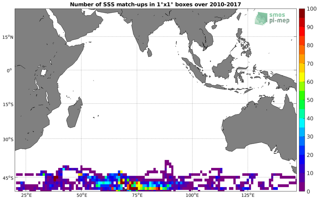
Figure 4: Number of SSS match-ups between Sea mammals SSS and the CCI SSS L4 Merged-OI v3.2 - 7-day running (ESA) SSS product for the Indian Ocean Pi-MEP region over 1°x1° boxes and for the full satellite product period.
