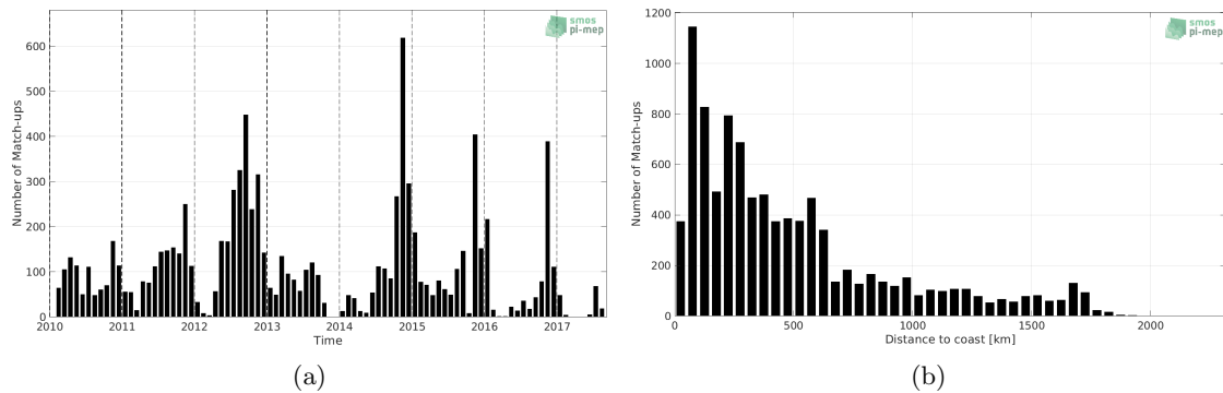
Figure 1: Number of match-ups between Sea mammals and CCI SSS L4 Merged-OI v3.2 - 7-day running (ESA) SSS as a function of time (a) and as function of the distance to coast (b) over the Indian Ocean Pi-MEP region and for the full satellite product period.
