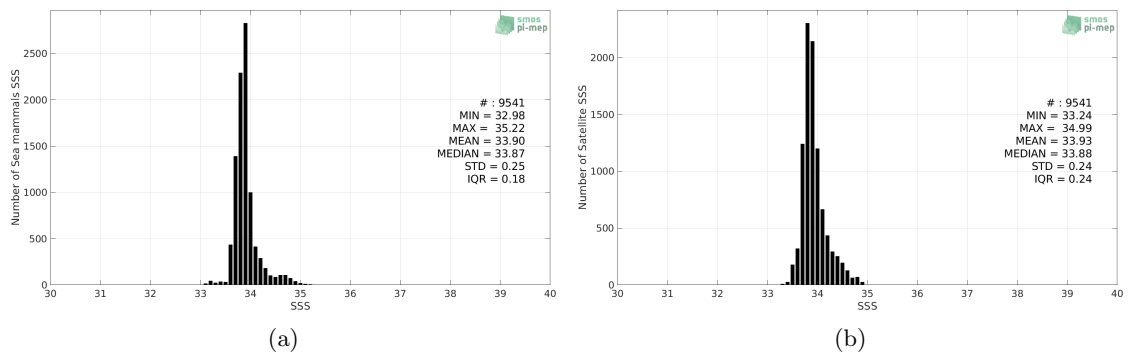
Figure 2: Histograms of SSS from Sea mammals (a) and CCI SSS L4 Merged-OI v3.2 - 7-day running (ESA) (b) considering all match-up pairs per bins of 0.1 over the Indian Ocean Pi-MEP region and for the full satellite product period.
