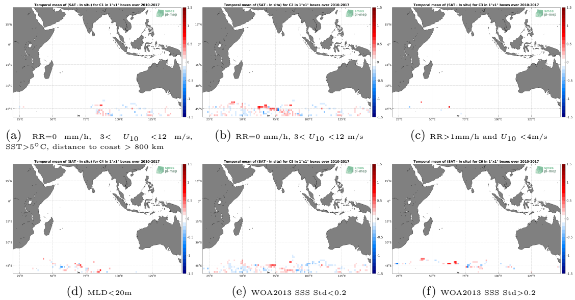
Figure 12: Temporal mean gridded over spatial boxes of size 1^{\circ}\times 1^{\circ} of \Delta\text{SSS} (CCI SSS L4 Merged-OI v3.2 - 7-day running (ESA) - Sea mammals) for 6 different subdatasets corresponding to: RR=0 mm/h, 3 < U_{10} < 12 m/s, SST > 5^{\circ}\text{C} , distance to coast > 800 km (a), RR=0 mm/h, 3 < U_{10} < 12 m/s (b), RR > 1 mm/h and U_{10} < 4 m/s (c), MLD < 20\text{m} (d), WOA2013 SSS Std < 0.2 (e), WOA2013 SSS Std > 0.2 (f).
