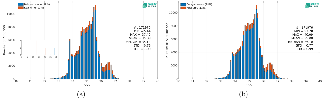
Figure 2: Histograms of SSS from Argo (a) and CCI SSS L4 Merged-OI v3.2 - 7-day running (ESA) (b) considering all match-up pairs per bins of 0.1 over the Indian Ocean Pi-MEP region and for the full satellite product period.
