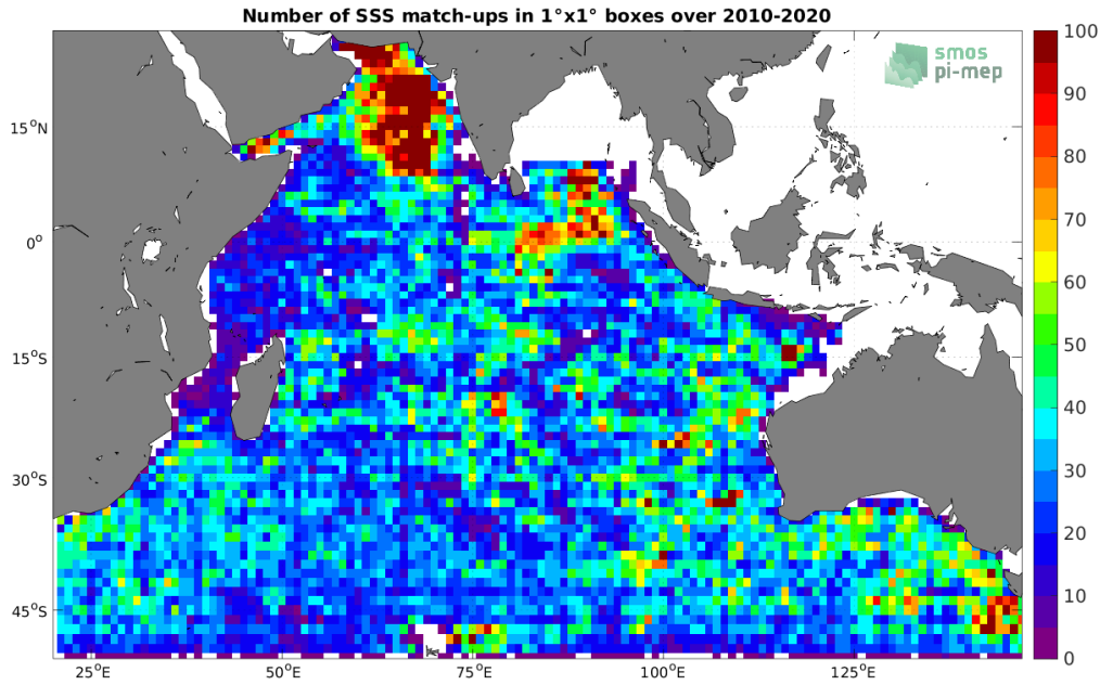
Figure 4: Number of SSS match-ups between Argo SSS and the CCI SSS L4 Merged-OI v3.2 - 7-day running (ESA) SSS product for the Indian Ocean Pi-MEP region over 1^\circ \times 1^\circ boxes and for the full satellite product period.
