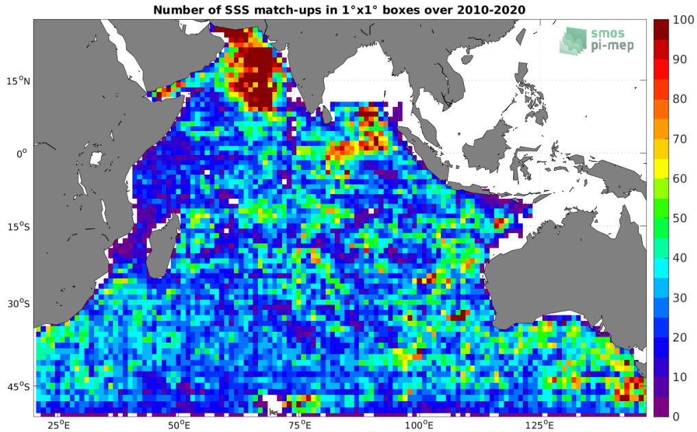
Figure 4: Number of SSS match-ups between Argo SSS and the CCI SSS L4 Merged-OI v3.2 - 7-day running (ESA) SSS product for the Indian Ocean Pi-MEP region over 1^\circ \times 1^\circ boxes and for the full satellite product period.
