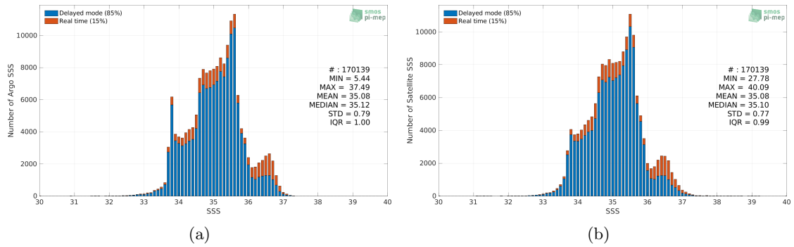
Figure 2: Histograms of SSS from Argo (a) and CCI SSS L4 Merged-OI v3.2 - 7-day running (ESA) (b) considering all match-up pairs per bins of 0.1 over the Indian Ocean Pi-MEP region and for the full satellite product period.
