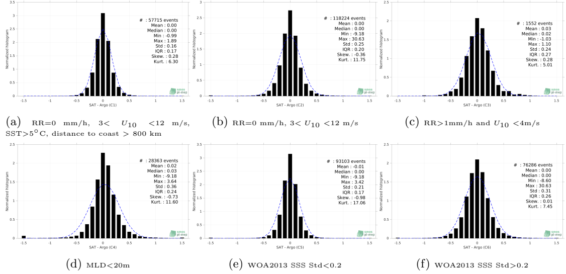
Figure 13: Normalized histogram of \Delta SSS (CCI SSS L4 Merged-OI v3.2 - 7-day running (ESA) - Argo) for 6 different subdatasets corresponding to: RR=0 mm/h, 3 < U_{10} < 12 m/s, SST > 5°C, distance to coast > 800 km (a), RR=0 mm/h, 3 < U_{10} < 12 m/s (b), RR > 1mm/h and U_{10} < 4 m/s (c), MLD < 20m (d), WOA2013 SSS Std < 0.2 (e), WOA2013 SSS Std > 0.2 (f).
