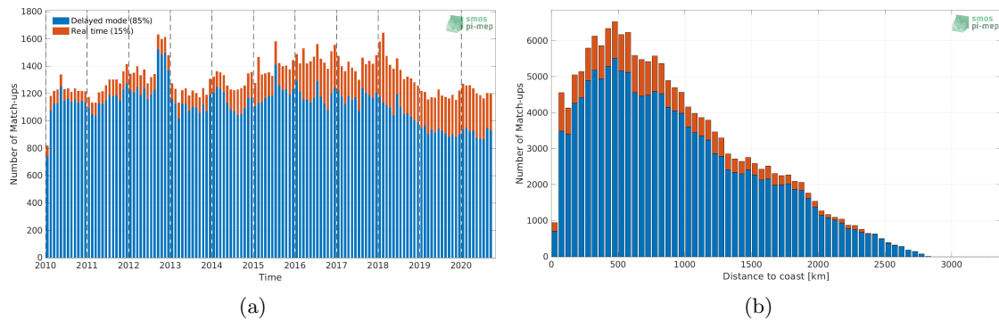
Figure 1: Number of match-ups between Argo and CCI SSS L4 Merged-OI v3.2 - 7-day running (ESA) SSS as a function of time (a) and as function of the distance to coast (b) over the Indian Ocean Pi-MEP region and for the full satellite product period.
