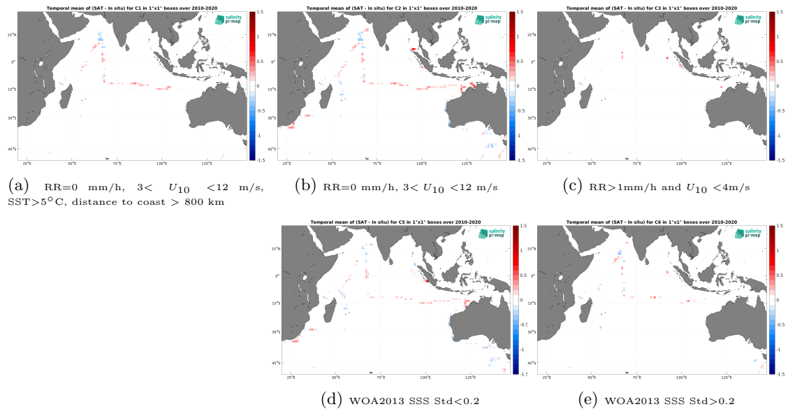
Figure 12: Temporal mean gridded over spatial boxes of size 1^\circ \times 1^\circ of \Delta SSS (CCI SSS L4 Merged-OI v3.2 - 30-day running (ESA) - TSG (SAMOS)) for 5 different subdatasets corresponding to:RR=0 mm/h, 3 < U_{10} < 12 m/s, SST >5^\circ C, distance to coast > 800 km (a), RR=0 mm/h, 3 < U_{10} < 12 m/s (b), RR >1 mm/h and U_{10} < 4 m/s (c), WOA2013 SSS Std <0.2 (d), WOA2013 SSS Std >0.2 (e).
