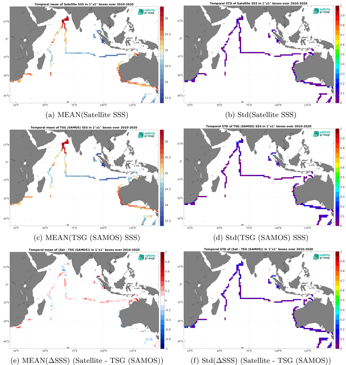
Figure 6: Temporal mean (left) and Std (right) of SSS from CCI SSS L4 Merged-OI v3.2 - 30-day running (ESA) (top), TSG (SAMOS) (middle), and of \Delta SSS (Satellite - TSG (SAMOS)). Only match-up pairs are used to generate these maps.
