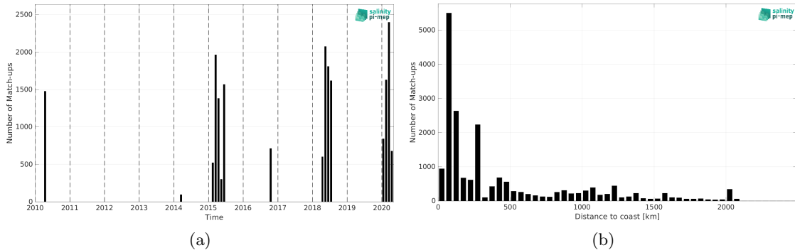
Figure 1: Number of match-ups between TSG (SAMOS) and CCI SSS L4 Merged-OI v3.2 - 30-day running (ESA) SSS as a function of time (a) and as function of the distance to coast (b) over the Indian Ocean Pi-MEP region and for the full satellite product period.
