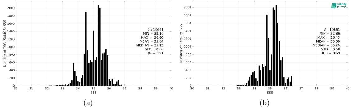
Figure 2: Histograms of SSS from TSG (SAMOS) (a) and CCI SSS L4 Merged-OI v3.2 - 30-day running (ESA) (b) considering all match-up pairs per bins of 0.1 over the Indian Ocean Pi-MEP region and for the full satellite product period.
