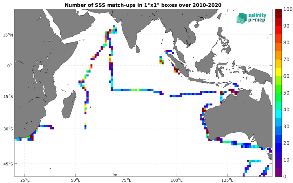
Figure 4: Number of SSS match-ups between TSG (SAMOS) SSS and the CCI SSS L4 Merged-OI v3.2 - 30-day running (ESA) SSS product for the Indian Ocean Pi-MEP region over 1^\circ \times 1^\circ boxes and for the full satellite product period.
