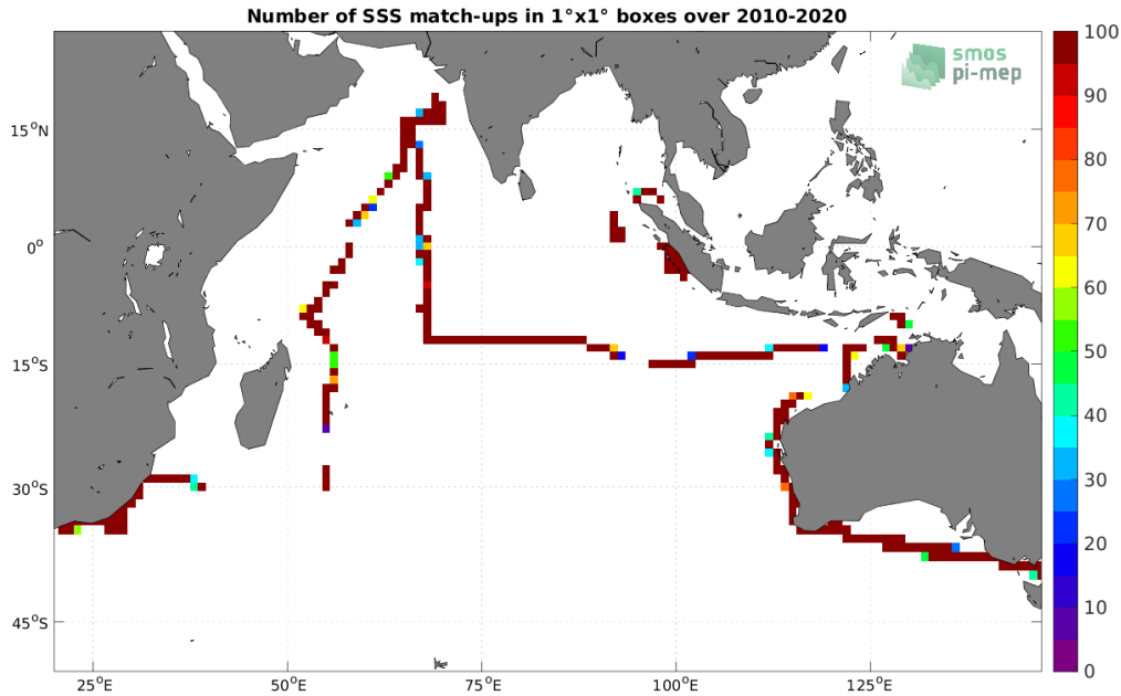
Figure 4: Number of SSS match-ups between TSG (SAMOS) SSS and the CCI SSS L4 Merged-OI v3.2 - 30-day running (ESA) SSS product for the Indian Ocean Pi-MEP region over 1^\circ \times 1^\circ boxes and for the full satellite product period.
