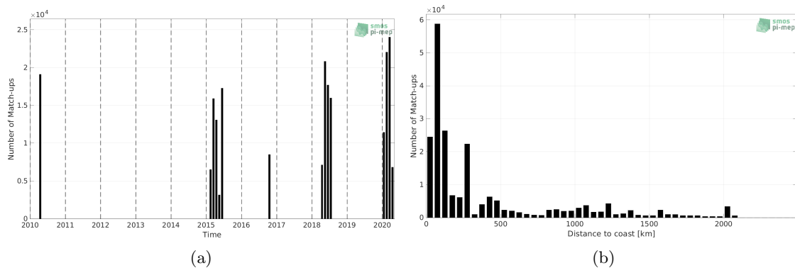
Figure 1: Number of match-ups between TSG (SAMOS) and CCI SSS L4 Merged-OI v3.2 - 30-day running (ESA) SSS as a function of time (a) and as function of the distance to coast (b) over the Indian Ocean Pi-MEP region and for the full satellite product period.
