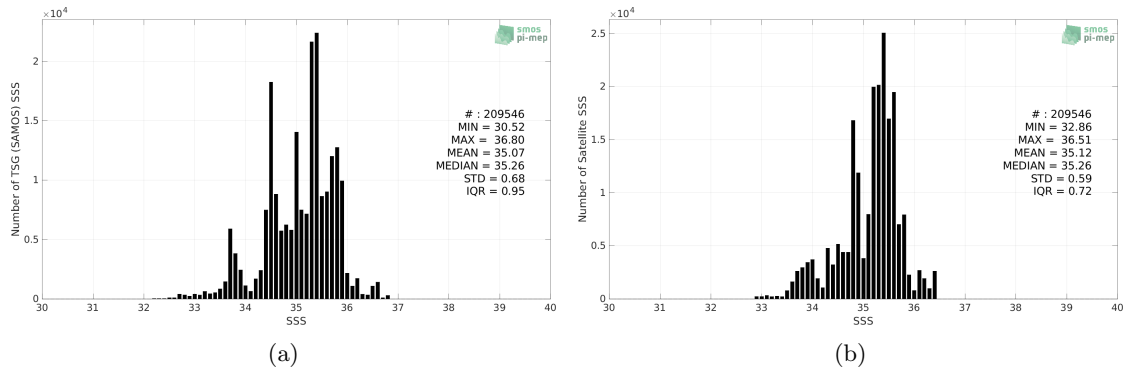
Figure 2: Histograms of SSS from TSG (SAMOS) (a) and CCI SSS L4 Merged-OI v3.2 - 30-day running (ESA) (b) considering all match-up pairs per bins of 0.1 over the Indian Ocean Pi-MEP region and for the full satellite product period.
