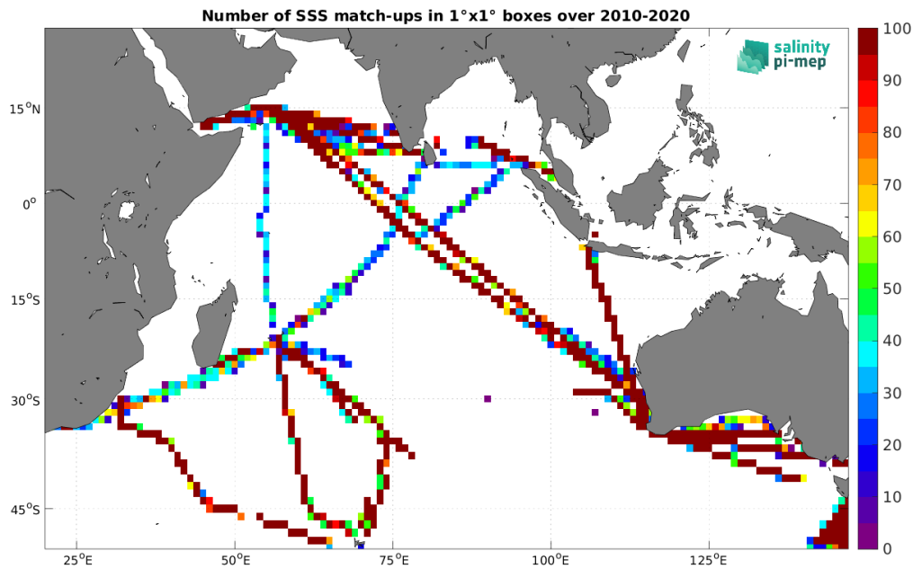
Figure 4: Number of SSS match-ups between TSG (LEGOS-DM) SSS and the CCI SSS L4 Merged-OI v3.2 - 30-day running (ESA) SSS product for the Indian Ocean Pi-MEP region over 1^\circ \times 1^\circ boxes and for the full satellite product period.
