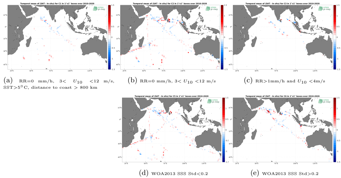
Figure 12: Temporal mean gridded over spatial boxes of size 1^\circ \times 1^\circ of \Delta SSS (CCI SSS L4 Merged-OI v3.2 - 30-day running (ESA) - TSG (LEGOS-DM)) for 5 different subdatasets corresponding to:RR=0 mm/h, 3 < U_{10} < 12 m/s, SST >5^\circ C, distance to coast > 800 km (a), RR=0 mm/h, 3 < U_{10} < 12 m/s (b), RR >1 mm/h and U_{10} < 4 m/s (c), WOA2013 SSS Std <0.2 (d), WOA2013 SSS Std >0.2 (e).
