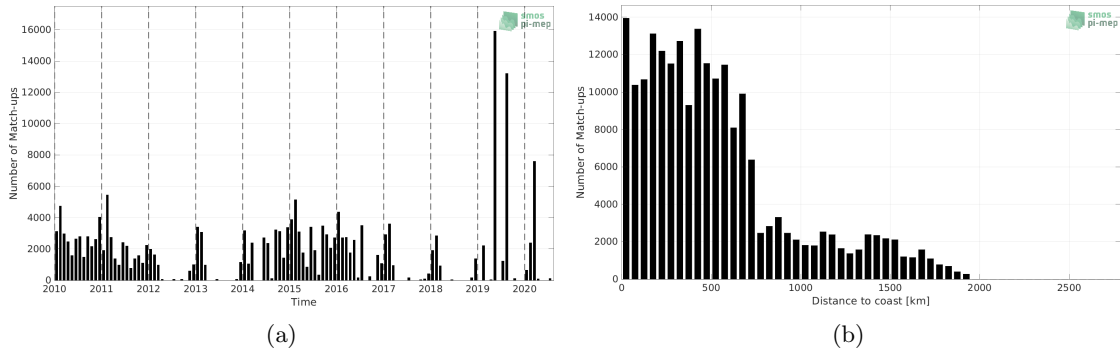
Figure 1: Number of match-ups between TSG (LEGOS-DM) and CCI SSS L4 Merged-OI v3.2 - 30-day running (ESA) SSS as a function of time (a) and as function of the distance to coast (b) over the Indian Ocean Pi-MEP region and for the full satellite product period.
