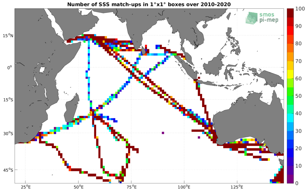
Figure 4: Number of SSS match-ups between TSG (LEGOS-DM) SSS and the CCI SSS L4 Merged-OI v3.2 - 30-day running (ESA) SSS product for the Indian Ocean Pi-MEP region over 1^\circ \times 1^\circ boxes and for the full satellite product period.
