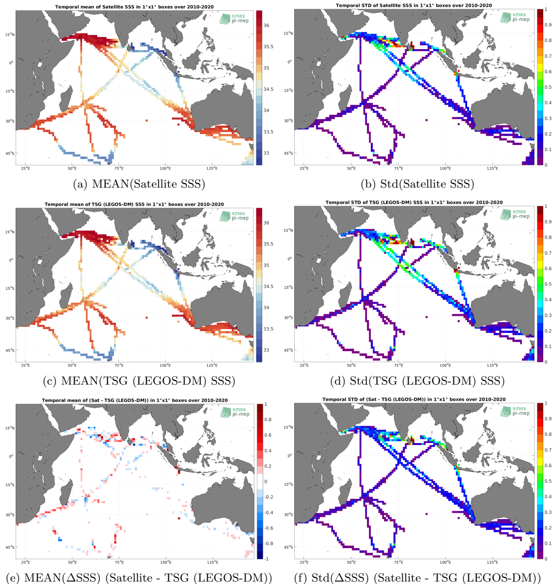
Figure 6: Temporal mean (left) and Std (right) of SSS from CCI SSS L4 Merged-OI v3.2 - 30-day running (ESA) (top), TSG (LEGOS-DM) (middle), and of \Delta SSS (Satellite - TSG (LEGOS-DM)). Only match-up pairs are used to generate these maps.
