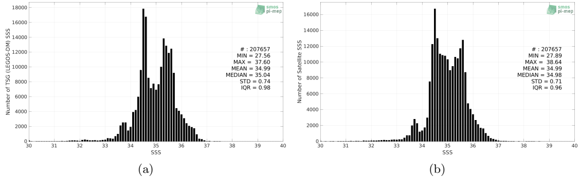
Figure 2: Histograms of SSS from TSG (LEGOS-DM) (a) and CCI SSS L4 Merged-OI v3.2 - 30-day running (ESA) (b) considering all match-up pairs per bins of 0.1 over the Indian Ocean Pi-MEP region and for the full satellite product period.
