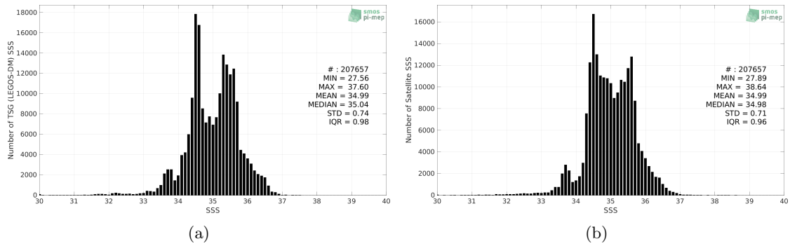
Figure 2: Histograms of SSS from TSG (LEGOS-DM) (a) and CCI SSS L4 Merged-OI v3.2 - 30-day running (ESA) (b) considering all match-up pairs per bins of 0.1 over the Indian Ocean Pi-MEP region and for the full satellite product period.
