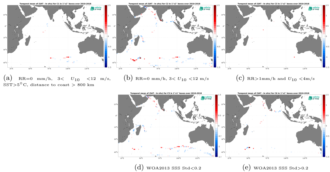
Figure 12: Temporal mean gridded over spatial boxes of size 1^\circ \times 1^\circ of \Delta\text{SSS} (CCI SSS L4 Merged-OI v3.2 - 30-day running (ESA) - TSG (GOSUD-Sailing-ship)) for 5 different subdatasets corresponding to:RR=0 mm/h, 3 < U_{10} < 12 m/s, SST >5^\circ\text{C} , distance to coast > 800 km (a), RR=0 mm/h, 3 < U_{10} < 12 m/s (b), RR >1 mm/h and U_{10} < 4 m/s (c), WOA2013 SSS Std <0.2 (d), WOA2013 SSS Std >0.2 (e).
