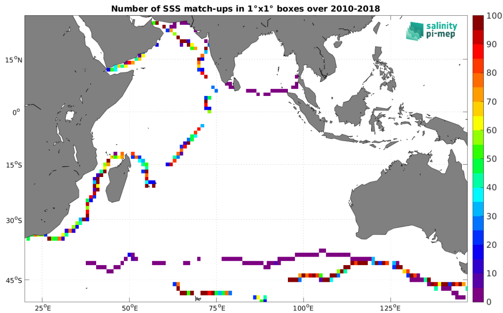
Figure 4: Number of SSS match-ups between TSG (GOSUD-Sailing-ship) SSS and the CCI SSS L4 Merged-OI v3.2 - 30-day running (ESA) SSS product for the Indian Ocean Pi-MEP region over 1^\circ \times 1^\circ boxes and for the full satellite product period.
