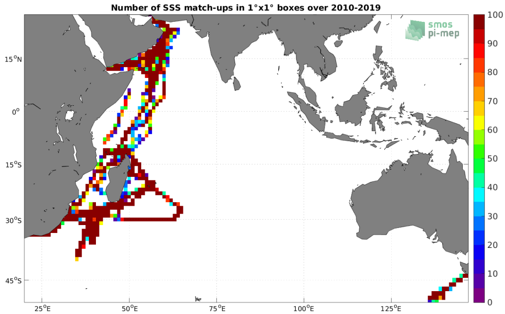
Figure 4: Number of SSS match-ups between TSG (GOSUD-Research-vessel) SSS and the CCI SSS L4 Merged-OI v3.2 - 30-day running (ESA) SSS product for the Indian Ocean Pi-MEP region over 1^\circ \times 1^\circ boxes and for the full satellite product period.
