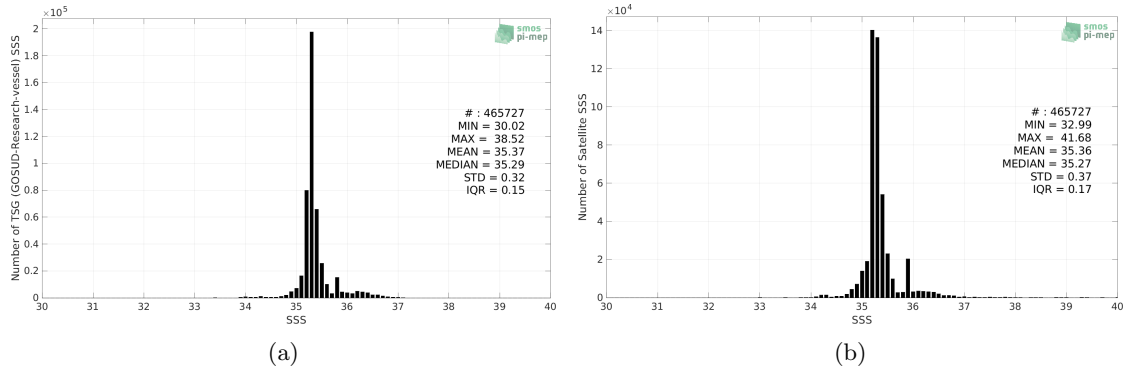
Figure 2: Histograms of SSS from TSG (GOSUD-Research-vessel) (a) and CCI SSS L4 Merged-OI v3.2 - 30-day running (ESA) (b) considering all match-up pairs per bins of 0.1 over the Indian Ocean Pi-MEP region and for the full satellite product period.
