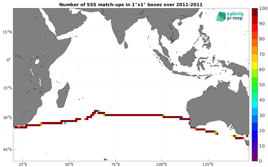
Figure 4: Number of SSS match-ups between TSG (CSIC-UTM) SSS and the CCI SSS L4 Merged-OI v3.2 - 30-day running (ESA) SSS product for the Indian Ocean Pi-MEP region over 1^\circ \times 1^\circ boxes and for the full satellite product period.
