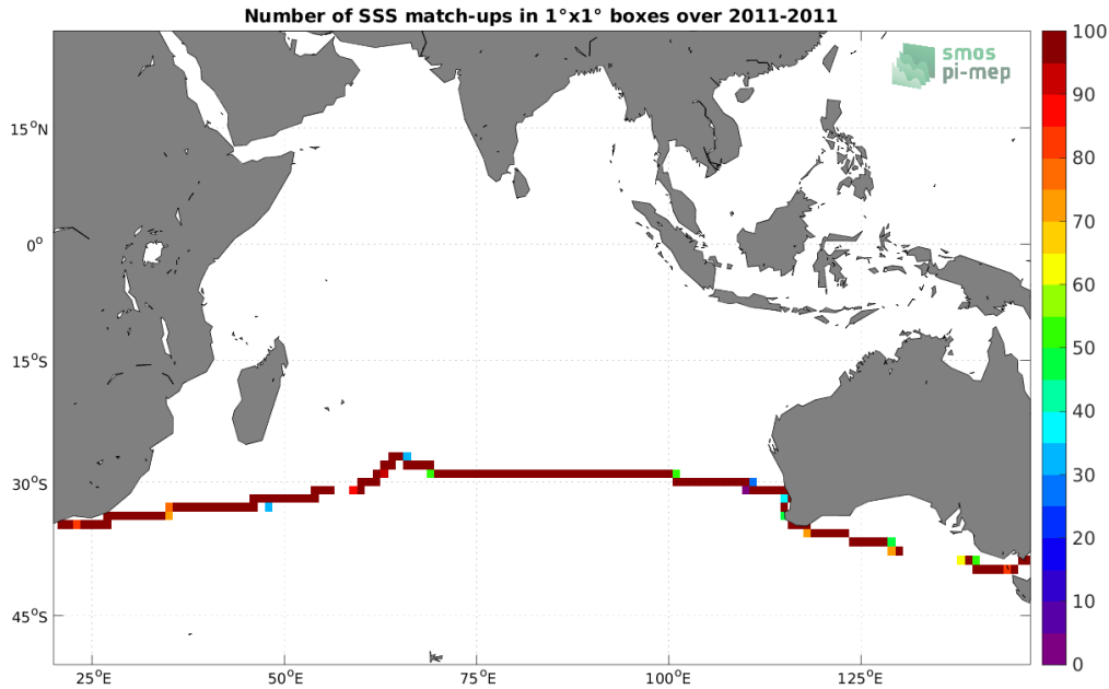
Figure 4: Number of SSS match-ups between TSG (CSIC-UTM) SSS and the CCI SSS L4 Merged-OI v3.2 - 30-day running (ESA) SSS product for the Indian Ocean Pi-MEP region over 1^\circ \times 1^\circ boxes and for the full satellite product period.
