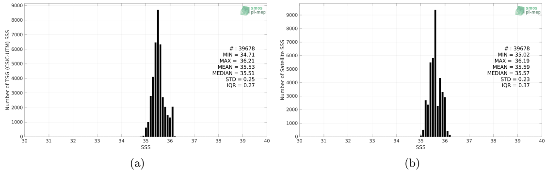
Figure 2: Histograms of SSS from TSG (CSIC-UTM) (a) and CCI SSS L4 Merged-OI v3.2 - 30-day running (ESA) (b) considering all match-up pairs per bins of 0.1 over the Indian Ocean Pi-MEP region and for the full satellite product period.
