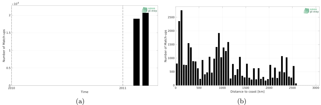
Figure 1: Number of match-ups between TSG (CSIC-UTM) and CCI SSS L4 Merged-OI v3.2 - 30-day running (ESA) SSS as a function of time (a) and as function of the distance to coast (b) over the Indian Ocean Pi-MEP region and for the full satellite product period.
