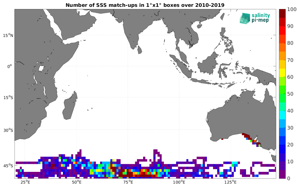
Figure 4: Number of SSS match-ups between Marine mammals SSS and the CCI SSS L4 Merged-OI v3.2 - 30-day running (ESA) SSS product for the Indian Ocean Pi-MEP region over 1^\circ \times 1^\circ boxes and for the full satellite product period.
