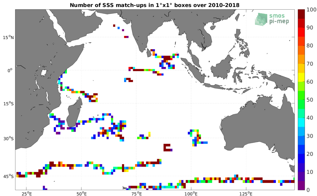
Figure 3: Number of SSS match-ups between Surface drifters SSS and the CCI SSS L4 Merged-OI v3.2 - 30-day running (ESA) SSS product for the Indian Ocean Pi-MEP region over 1^\circ \times 1^\circ boxes and for the full satellite product period.
