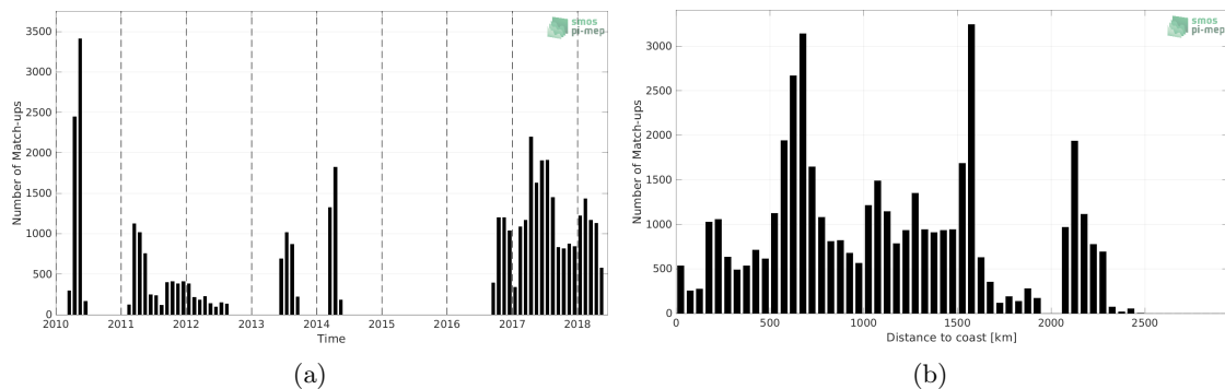
Figure 1: Number of match-ups between Surface drifters and CCI SSS L4 Merged-OI v3.2 - 30-day running (ESA) SSS as a function of time (a) and as function of the distance to coast (b) over the Indian Ocean Pi-MEP region and for the full satellite product period.
