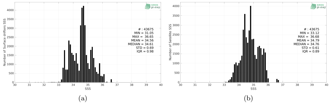
Figure 2: Histograms of SSS from Surface drifters (a) and CCI SSS L4 Merged-OI v3.2 - 30-day running (ESA) (b) considering all match-up pairs per bins of 0.1 over the Indian Ocean Pi-MEP region and for the full satellite product period.
