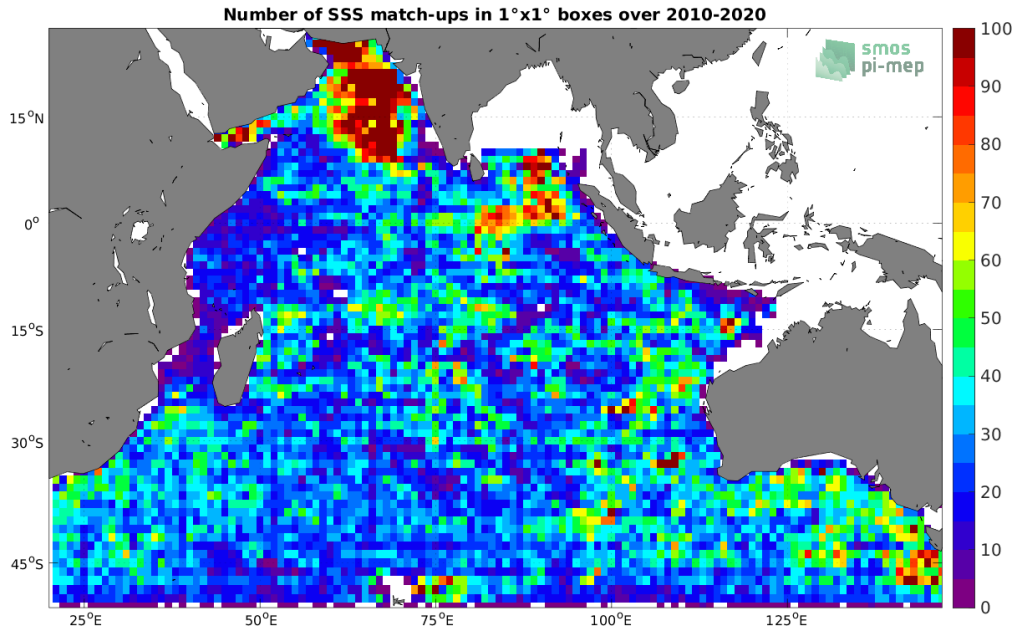
Figure 4: Number of SSS match-ups between Argo SSS and the CCI SSS L4 Merged-OI v3.2 - 30-day running (ESA) SSS product for the Indian Ocean Pi-MEP region over 1^\circ \times 1^\circ boxes and for the full satellite product period.
