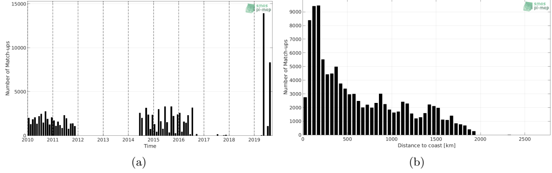
Figure 1: Number of match-ups between TSG (LEGOS-DM) and CCI SSS L4 Merged-OI v2.31 - 30-day running (ESA) SSS as a function of time (a) and as function of the distance to coast (b) over the Indian Ocean Pi-MEP region and for the full satellite product period.
