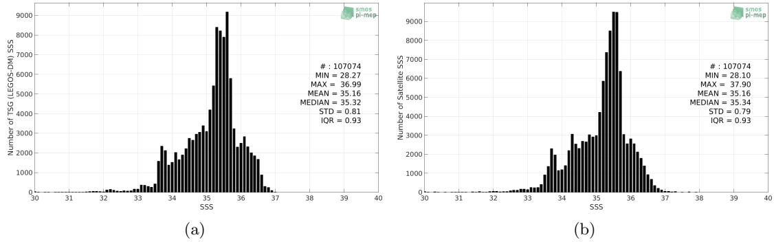
Figure 2: Histograms of SSS from TSG (LEGOS-DM) (a) and CCI SSS L4 Merged-OI v2.31 - 30-day running (ESA) (b) considering all match-up pairs per bins of 0.1 over the Indian Ocean Pi-MEP region and for the full satellite product period.
