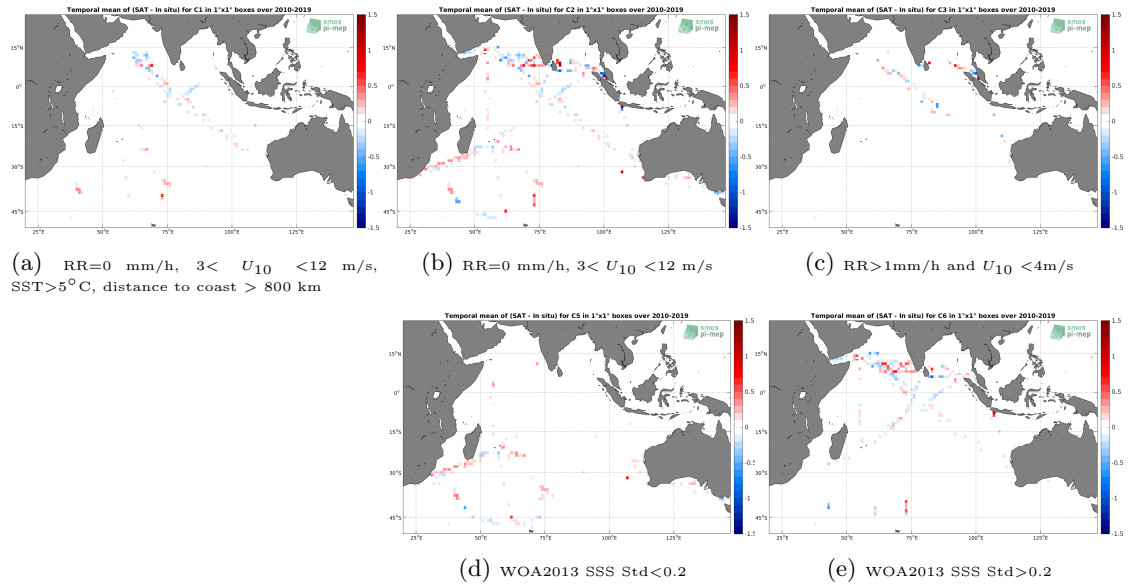
Figure 12: Temporal mean gridded over spatial boxes of size 1^\circ \times 1^\circ of \Delta SSS (CCI SSS L4 Merged-OI v2.31 - 30-day running (ESA) - TSG (LEGOS-DM)) for 5 different subdatasets corresponding to: RR=0 mm/h, 3 < U_{10} < 12 m/s, SST > 5^\circ C , distance to coast > 800 km (a), RR=0 mm/h, 3 < U_{10} < 12 m/s (b), RR > 1 mm/h and U_{10} < 4 m/s (c), WOA2013 SSS Std < 0.2 (d), WOA2013 SSS Std > 0.2 (e).
