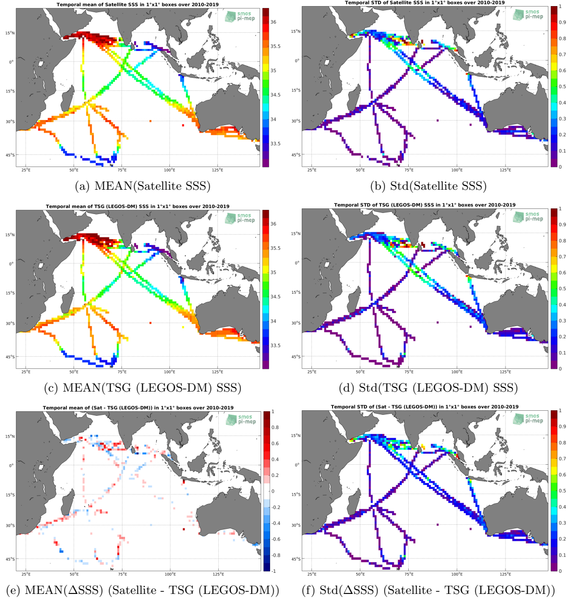
Figure 6: Temporal mean (left) and Std (right) of SSS from CCI SSS L4 Merged-OI v2.31 - 30-day running (ESA) (top), TSG (LEGOS-DM) (middle), and of \Delta SSS (Satellite - TSG (LEGOS-DM)). Only match-up pairs are used to generate these maps.
