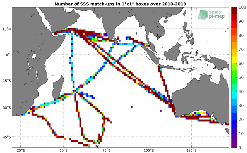
Figure 4: Number of SSS match-ups between TSG (LEGOS-DM) SSS and the CCI L4 Merged-OI v2.31 - 30-day running (ESA) SSS product for the Indian Ocean Pi-MEP region over 1°x1° boxes and for the full satellite product period.
