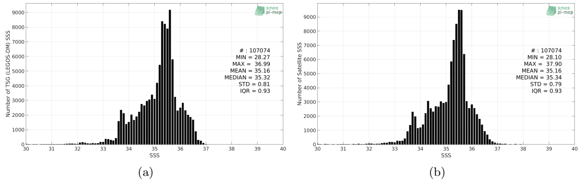
Figure 2: Histograms of SSS from TSG (LEGOS-DM) (a) and CCI L4 Merged-OI v2.31 - 30-day running (ESA) (b) considering all match-up pairs per bins of 0.1 over the Indian Ocean Pi-MEP region and for the full satellite product period.
