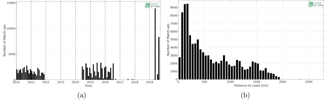
Figure 1: Number of match-ups between TSG (LEGOS-DM) and CCI L4 Merged-OI v2.31 - 30-day running (ESA) SSS as a function of time (a) and as function of the distance to coast (b) over the Indian Ocean Pi-MEP region and for the full satellite product period.
