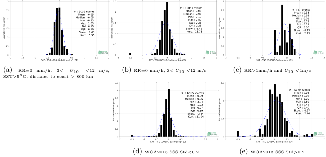
Figure 13: Normalized histogram of \Delta\text{SSS} (CCI L4 Merged-OI v2.31 - 30-day running (ESA) - TSG (GOSUD-Sailing-ship)) for 5 different subdatasets corresponding to: RR=0 mm/h, 3 < U_{10} < 12 m/s, SST > 5^\circ\text{C} , distance to coast > 800 km (a), RR=0 mm/h, 3 < U_{10} < 12 m/s (b), RR > 1\text{mm/h} and U_{10} < 4\text{m/s} (c), WOA2013 SSS Std < 0.2 (d), WOA2013 SSS Std > 0.2 (e).
