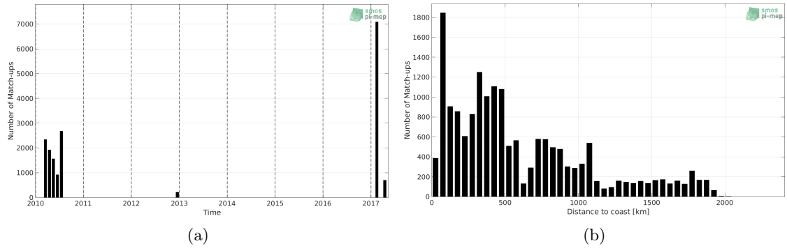
Figure 1: Number of match-ups between TSG (GOSUD-Sailing-ship) and CCI L4 Merged-OI v2.31 - 30-day running (ESA) SSS as a function of time (a) and as function of the distance to coast (b) over the Indian Ocean Pi-MEP region and for the full satellite product period.
