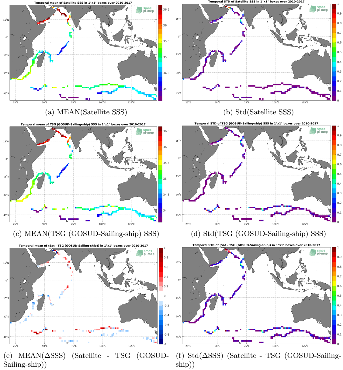
Figure 6: Temporal mean (left) and Std (right) of SSS from CCI L4 Merged-OI v2.31 - 30-day running (ESA) (top), TSG (GOSUD-Sailing-ship) (middle), and of \Delta SSS (Satellite - TSG (GOSUD-Sailing-ship)). Only match-up pairs are used to generate these maps.
