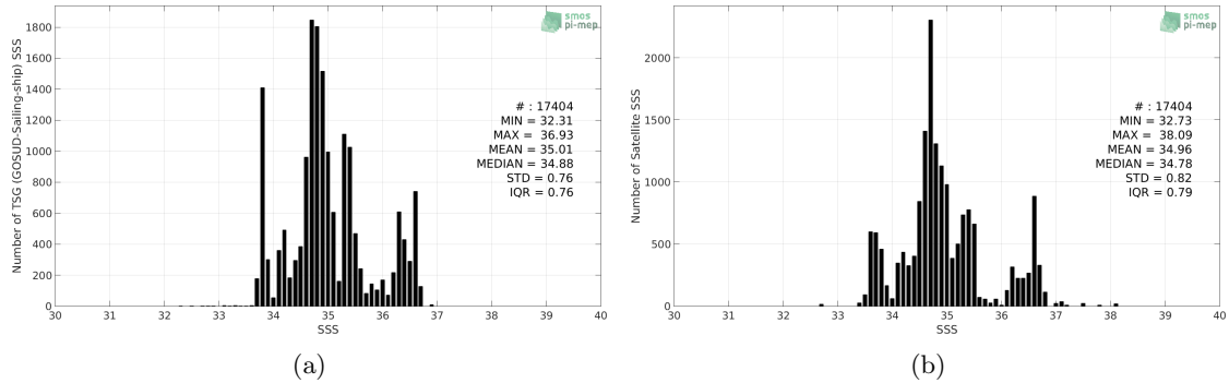
Figure 2: Histograms of SSS from TSG (GOSUD-Sailing-ship) (a) and CCI L4 Merged-OI v2.31 - 30-day running (ESA) (b) considering all match-up pairs per bins of 0.1 over the Indian Ocean Pi-MEP region and for the full satellite product period.
