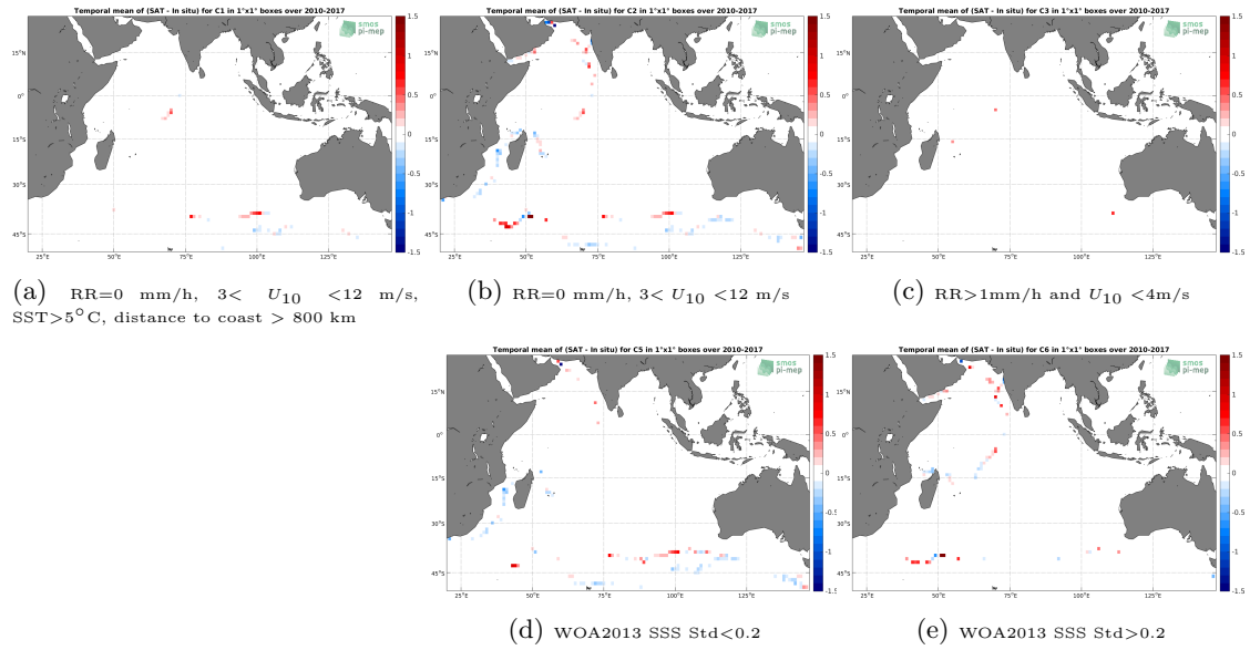
Figure 12: Temporal mean gridded over spatial boxes of size 1^\circ \times 1^\circ of \Delta SSS (CCI L4 Merged-OI v2.31 - 30-day running (ESA) - TSG (GOSUD-Sailing-ship)) for 5 different subdatasets corresponding to: RR=0 mm/h, 3 < U_{10} < 12 m/s, SST > 5^\circ C , distance to coast > 800 km (a), RR=0 mm/h, 3 < U_{10} < 12 m/s (b), RR > 1 mm/h and U_{10} < 4 m/s (c), WOA2013 SSS Std < 0.2 (d), WOA2013 SSS Std > 0.2 (e).
