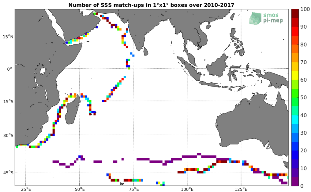
Figure 4: Number of SSS match-ups between TSG (GOSUD-Sailing-ship) SSS and the CCI L4 Merged-OI v2.31 - 30-day running (ESA) SSS product for the Indian Ocean Pi-MEP region over 1°x1° boxes and for the full satellite product period.
