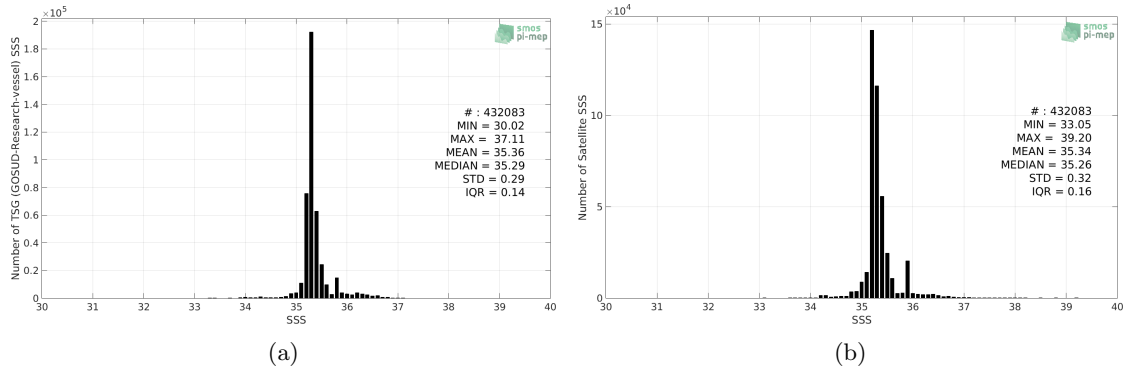
Figure 2: Histograms of SSS from TSG (GOSUD-Research-vessel) (a) and CCI L4 Merged-OI v2.31 - 30-day running (ESA) (b) considering all match-up pairs per bins of 0.1 over the Indian Ocean Pi-MEP region and for the full satellite product period.
