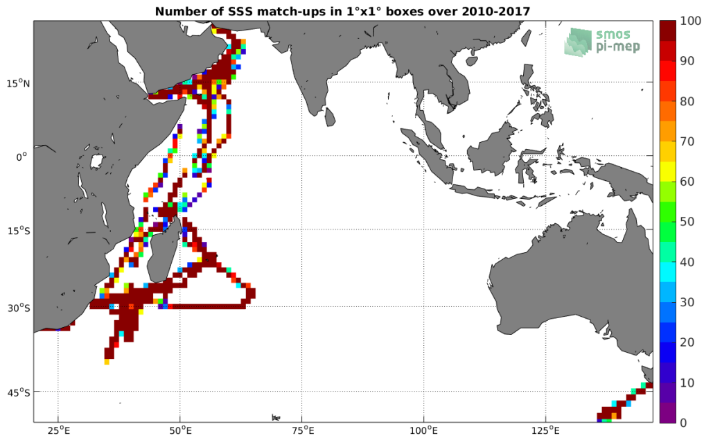
Figure 4: Number of SSS match-ups between TSG (GOSUD-Research-vessel) SSS and the CCI L4 Merged-OI v2.31 - 30-day running (ESA) SSS product for the Indian Ocean Pi-MEP region over 1°x1° boxes and for the full satellite product period.
